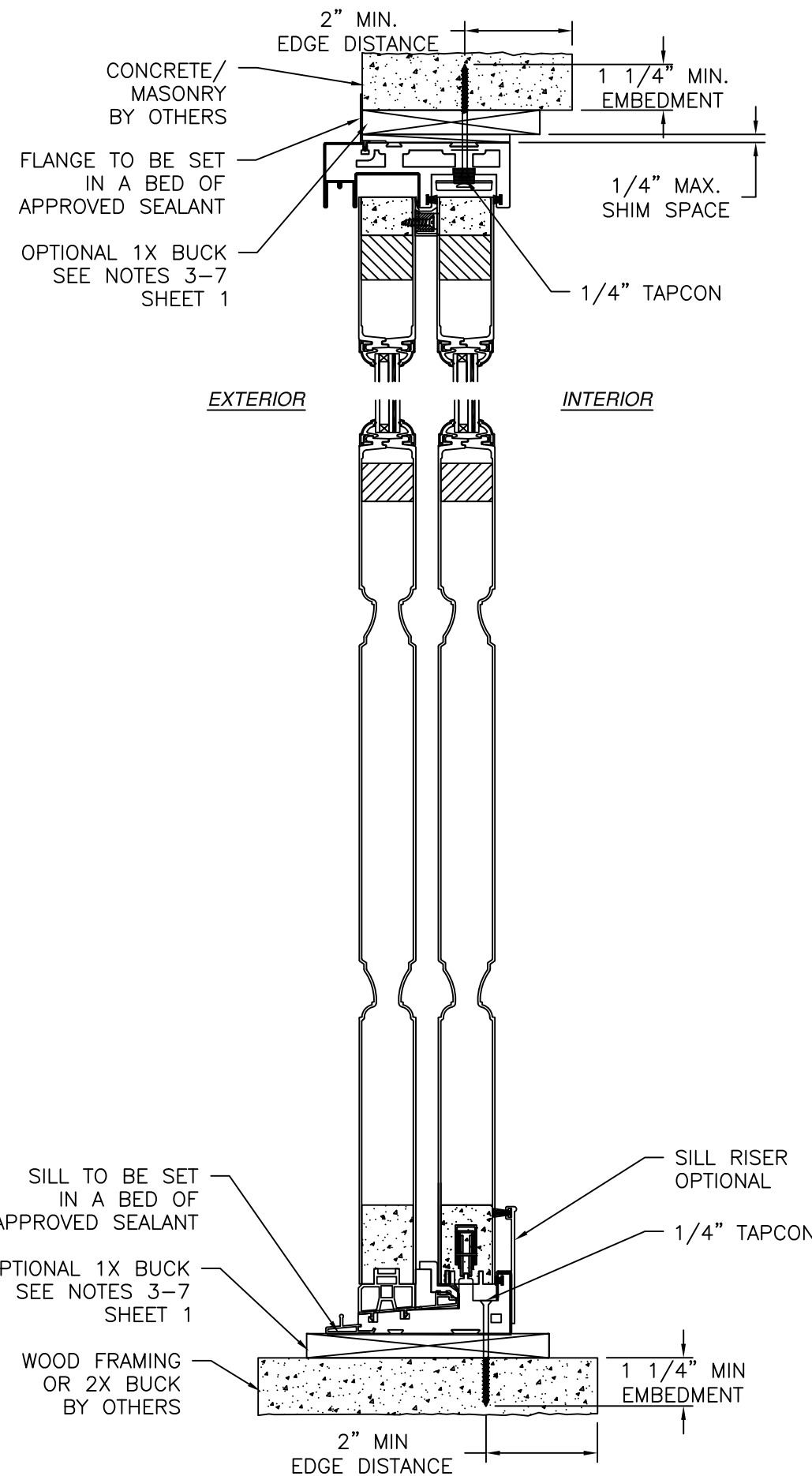
VERTICAL CROSS SECTION CONCRETE/MASONRY INSTALLATION
