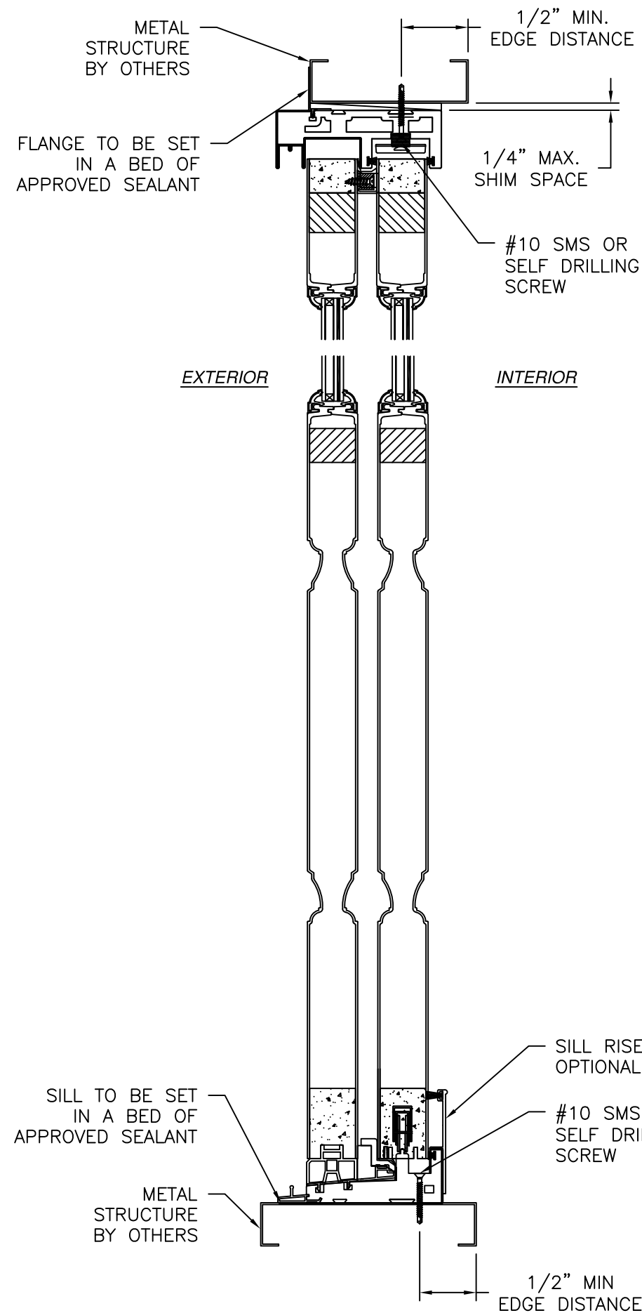
VERTICAL CROSS SECTION METAL STRUCTURE INSTALLATION
