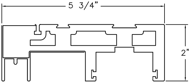
HEAD FOAM PVC CO-EX
