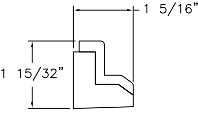
SILL WIND STOPPER FOAM EPDM
