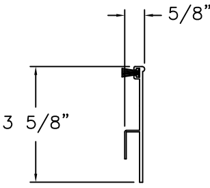
SILL RISER ALUMINUM
