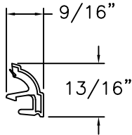
GLAZING BEAD PVC
