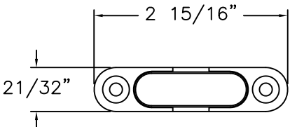
ANTI-LIFT STOPPER DIE CASTING
