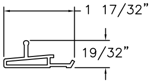
SCREEN TRACK ALUMINUM
