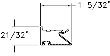
INTERLOCK STRIP FOAM PVC
