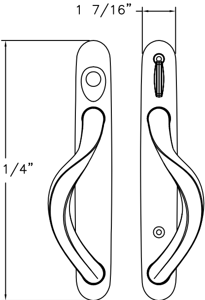
GLIDING HANDLE DIE CAST, STEEL
