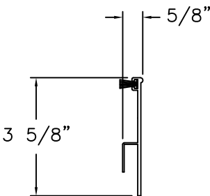
SILL RISER ALUMINUM
