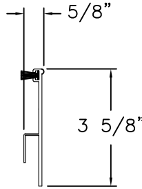
SILL RISER ALUMINUM
