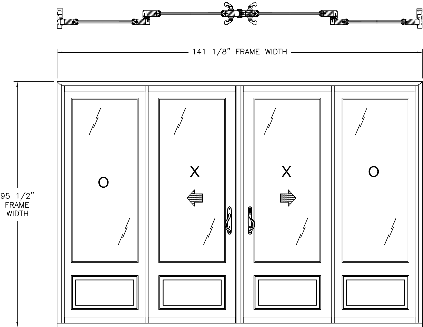
SERIES "SPLS" 8'0 FIBERGLASS SLIDING GLASS DOOR WITH 3/4" PANELS
