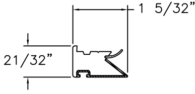
INTERLOCK STRIP FOAM PVC
