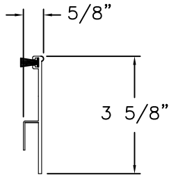
SILL RISER ALUMINUM
