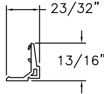
GLAZING BEAD PVC
