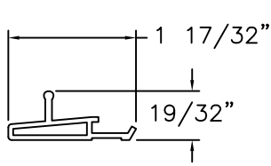
SCREEN TRACK ALUMINUM
