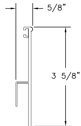
SILL RISER ALUMINUM
