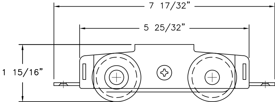
ADJUSTABLE ROLLER STAINLESS STEEL
