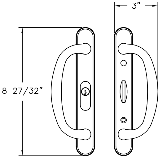
HANDLE SET DIE CASTING
