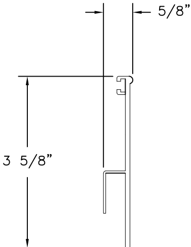
SILL RISER ALUMINUM
