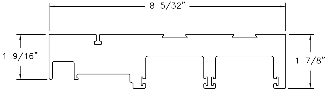
FRAME HEAD & JAMB FOAM PVC CO-EX
