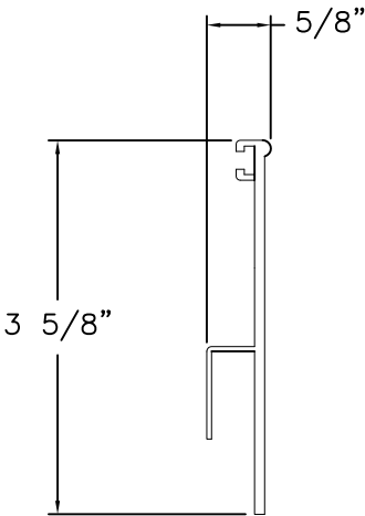
SILL RISER ALUMINUM
