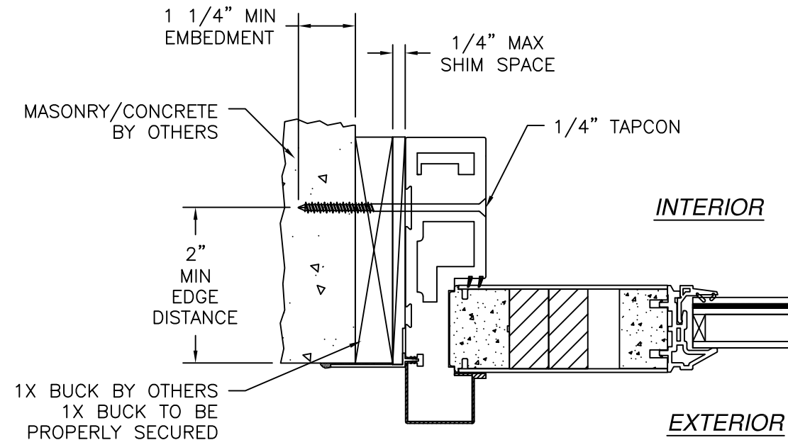
HORIZONTAL CROSS SECTION MASONRY/CONCRETE INSTALLATION
