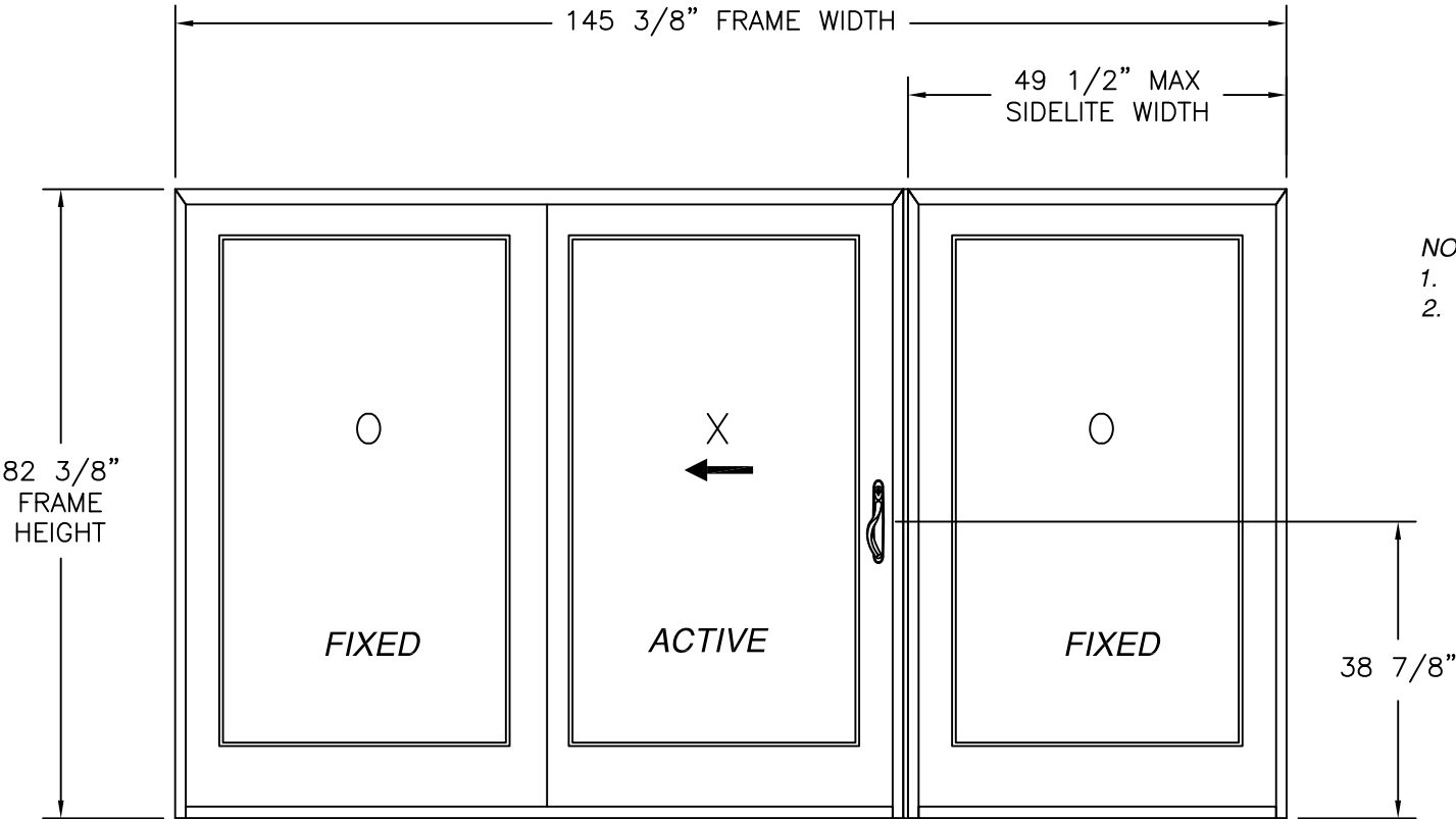
SERIES SRS GLIDING PATIO DOOR W/FIELD MULLION - 120611 IMPACT EXTERIOR VIEW
