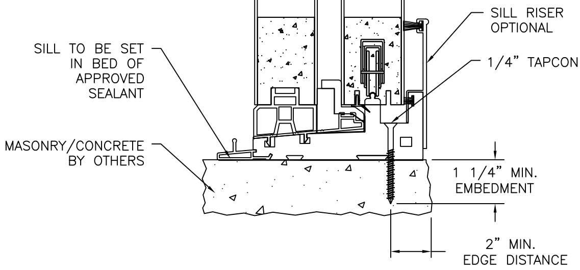
VERTICAL CROSS SECTION MASONRY/CONCRETE INSTALLATION DOOR SHOWN SIDELITE SIMILAR
