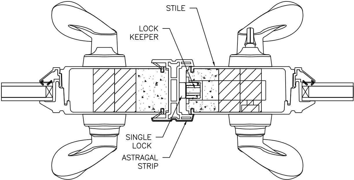
ASTRAGAL DETAIL
