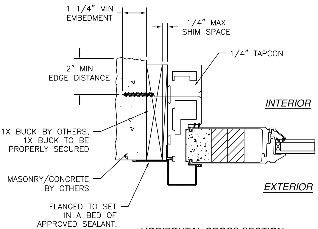
HORIZONTAL CROSS SECTION MASONRY/CONCRETE INSTALLATION
