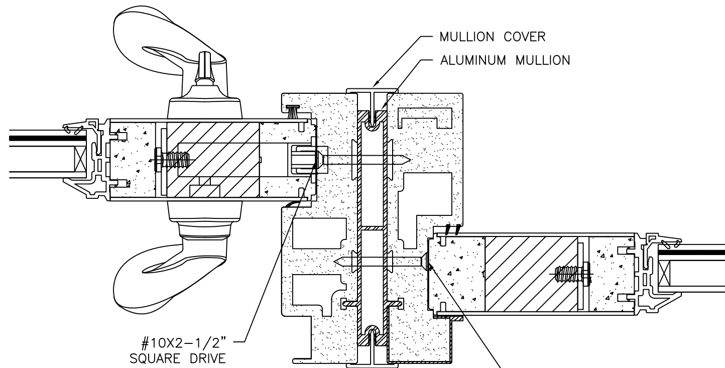
MULLION DETAIL
