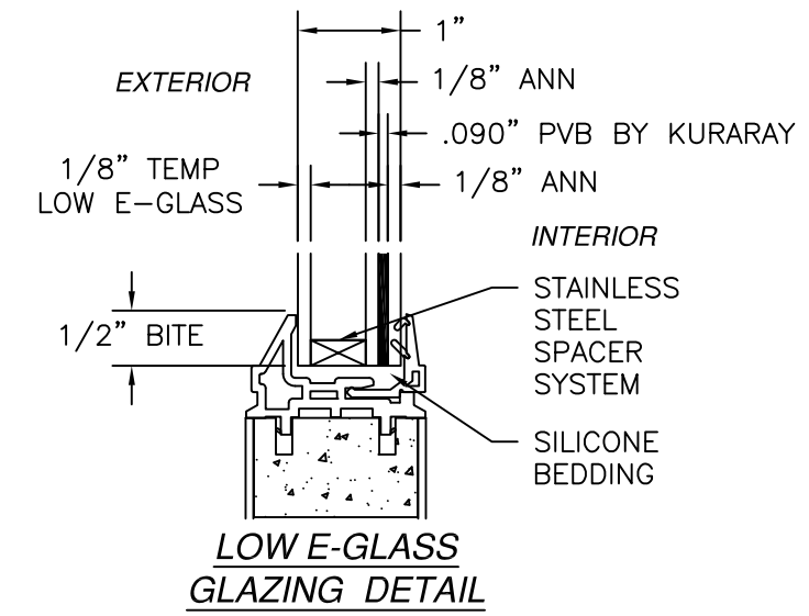
MINI-BLIND GLAZING DETAIL
