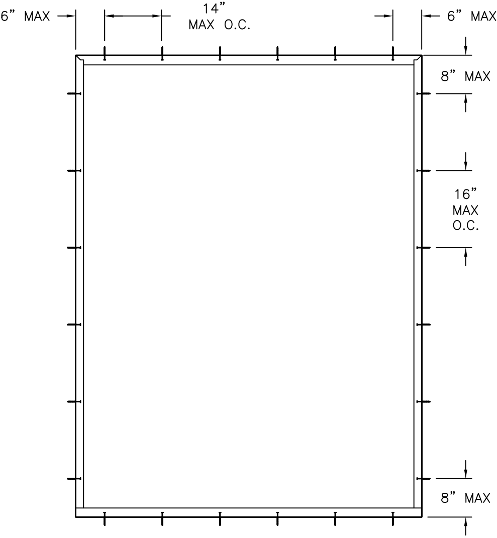
ANCHORING LAYOUT FOR OX AND XO CONFIGURATION EXTERIOR VIEW
