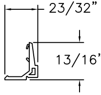
GLAZING BEAD PVC
