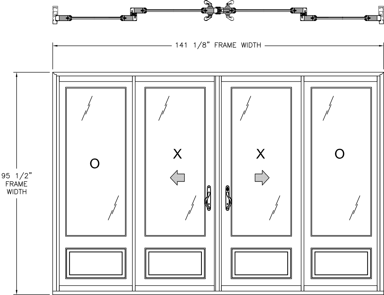
SERIES "SPLS" 8'0 FIBERGLASS SLIDING GLASS DOOR WITH 3/4" PANELS EXTERIOR VIEW
