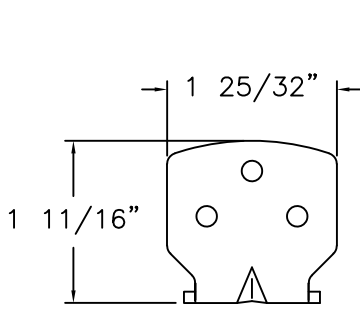
TOP BRACKET STAINLESS STEEL
