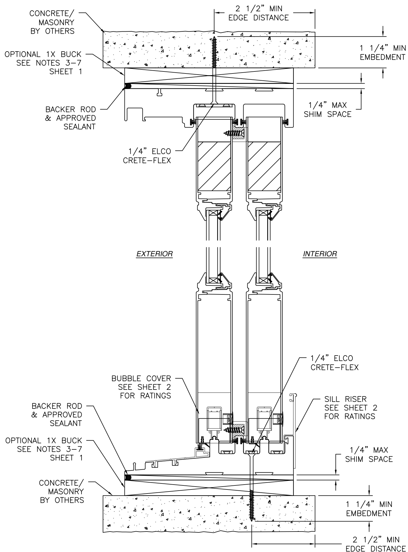
VERTICAL CROSS SECTION CONCRETE/MASONRY INSTALLATION
