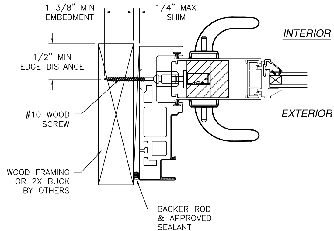
DOOR JAMB INSTALLATION DETAIL WOOD FRAMING OR 2X BUCK INSTALLATION
