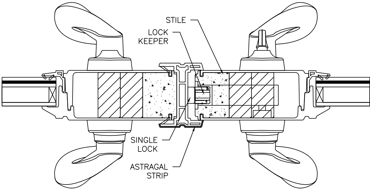
ASTRAGAL DETAIL
