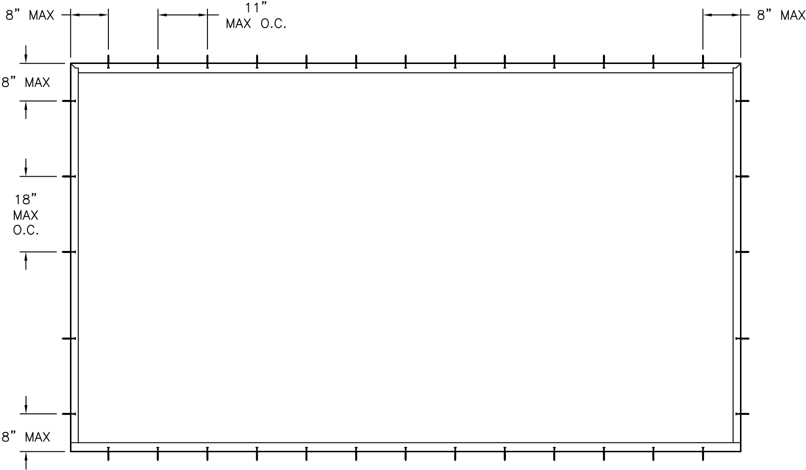
ANCHORING LAYOUT FOR DOUBLE W/SIDELITES EXTERIOR VIEW
