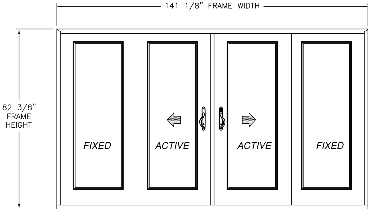
SERIES SPLS GLIDING PATIO DOOR - 120611 EXTERIOR VIEW
