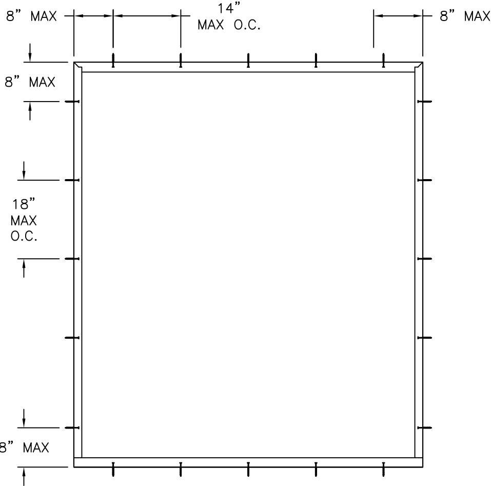
ANCHORING LAYOUT FOR SINGLE W/SIDELITE EXTERIOR VIEW
