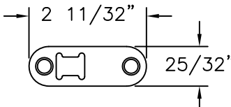
26 FLUSH BOLT GUIDE1 STAINLESS STEEL
