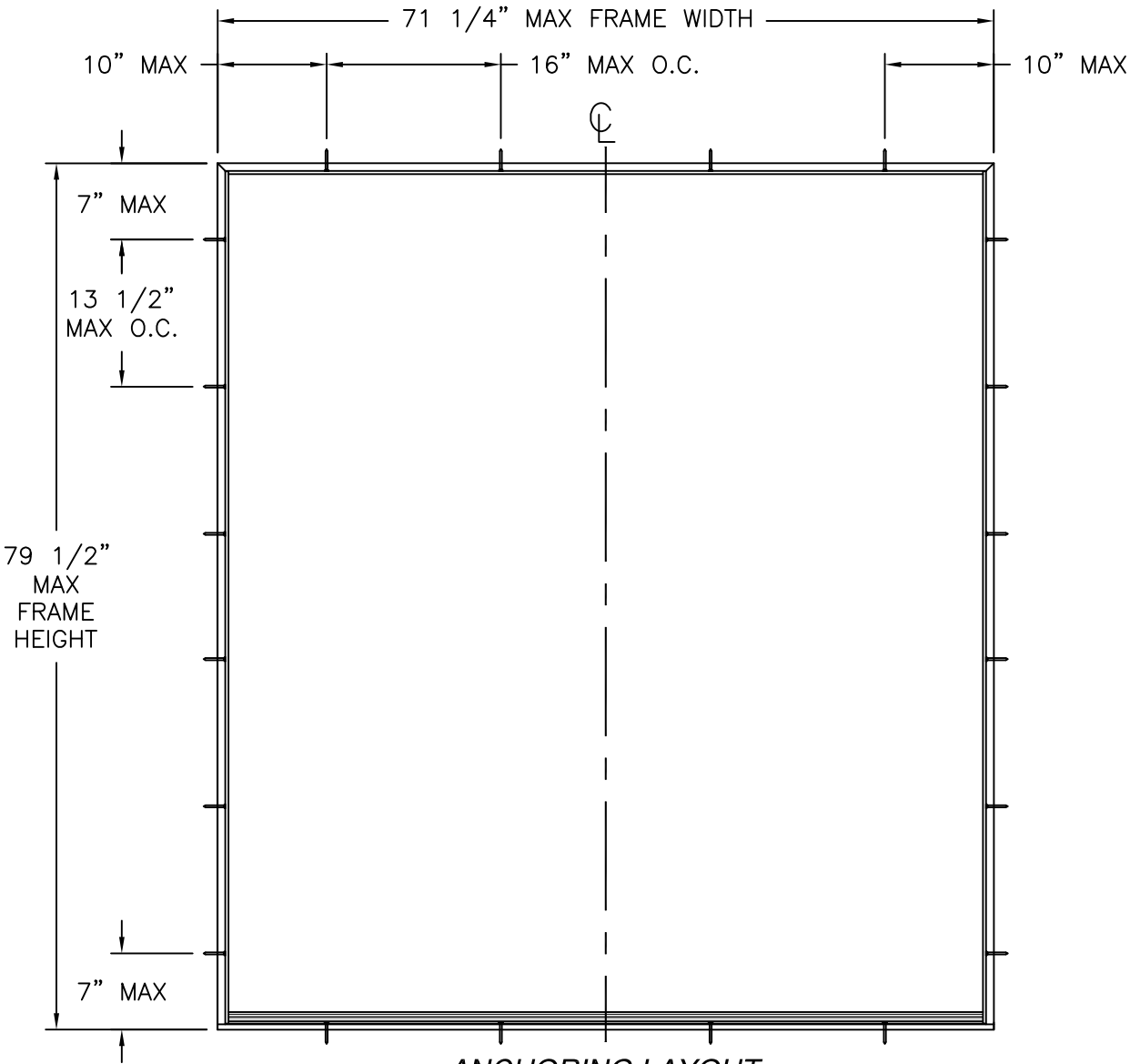
ANCHORING LAYOUT
