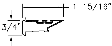
11 MEETING STILE INTERLOCK FOAM PVC CO-EX.
