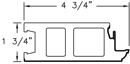
3 4 3/4" LOCK STILE PVC COMPONENT
