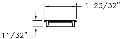
18 INTERIOR WEEPER ABS
