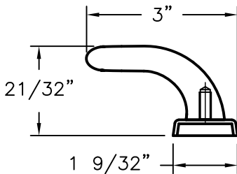
31 GLIDING HANDLE DIE CAST, STEEL
