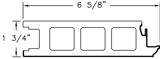
4 6 5/8" BOTTOM RAIL PVC COMPONENT
