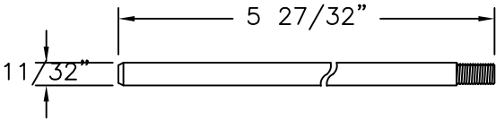
29 FLUSH BOLT BAR STAINLESS STEEL
