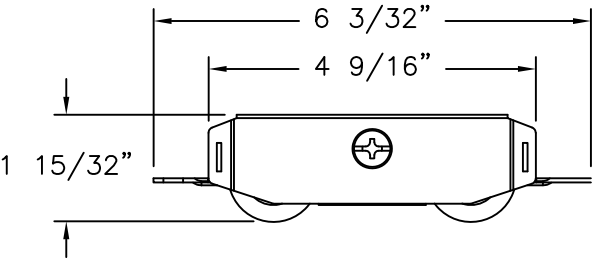
22 ADJUSTABLE ROLLER STAINLESS STEEL
