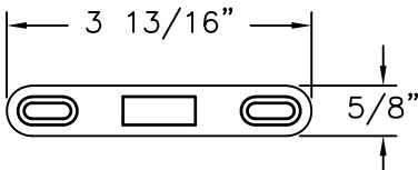
27 LOCK KEEPER DIE CASTING
