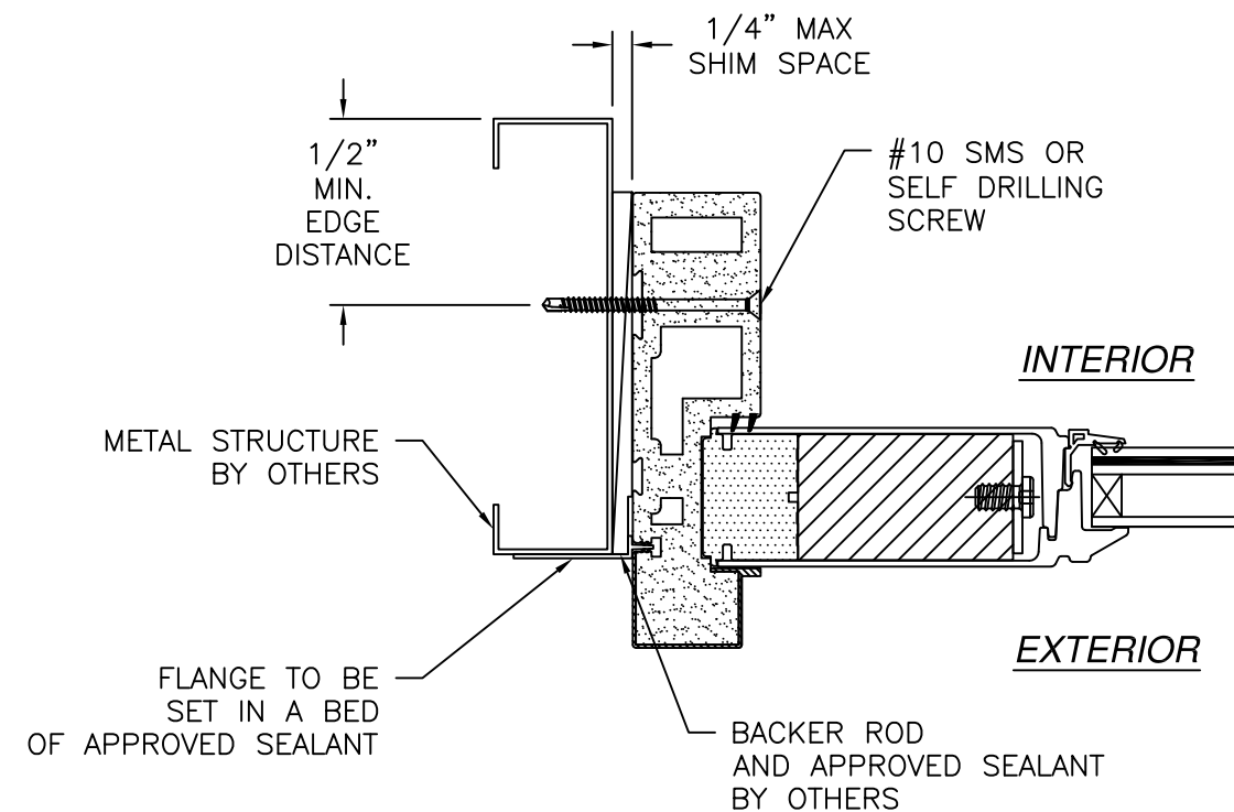
HORIZONTAL CROSS SECTION METAL STRUCTURE INSTALLATION
