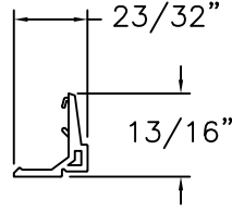
GLAZING BEAD PVC
