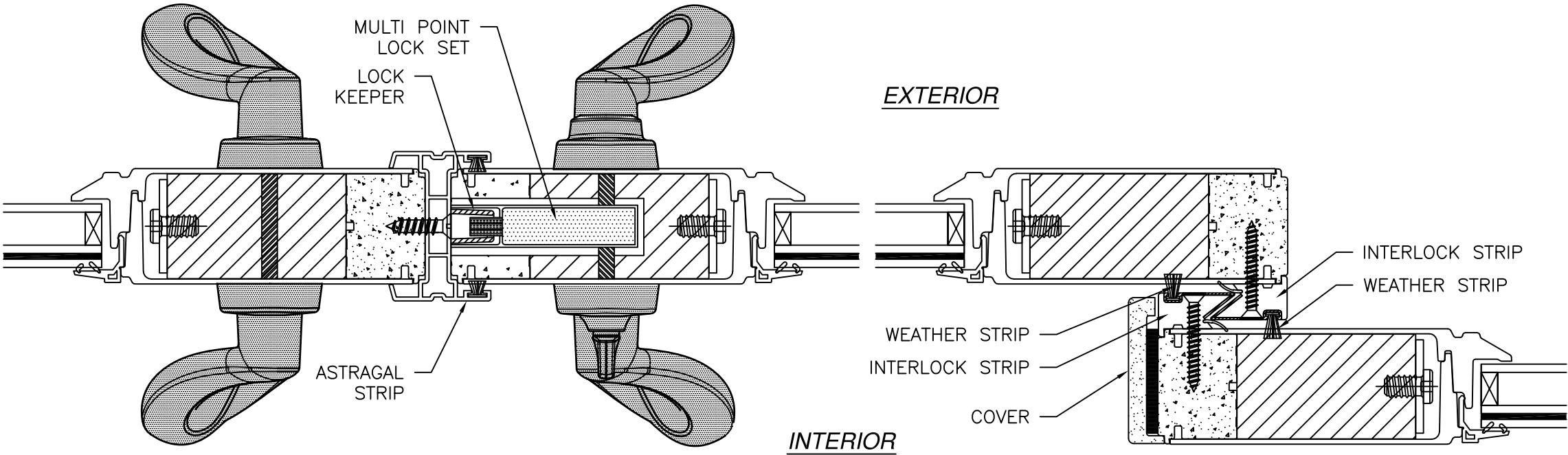
ASTRAGAL AND MEETING RAIL DETAIL
