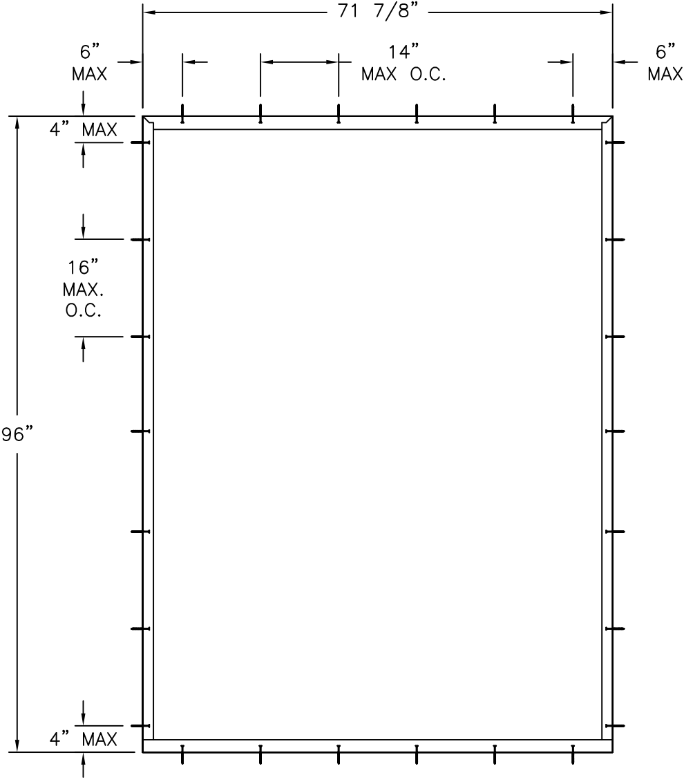
ANCHORING LAYOUT FOR OX OR XO EXTERIOR VIEW
