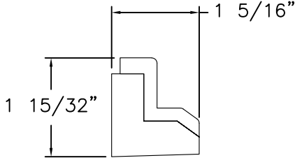
WIND STOPPER (B) FOAM EPDM
