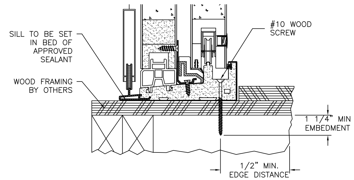
VERTICAL CROSS SECTION DOOR SHOWN, SIDELITE SIMILAR 2X BUCK/WOOD FRAMING INSTALLATION
