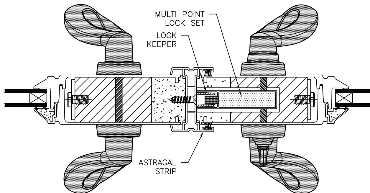
ASTRAGAL DETAIL
