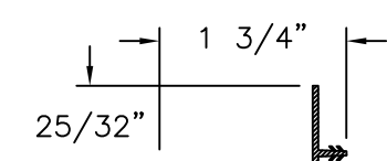
FRAME FIN EXTRUDED RIGID PVC .051" THICK
