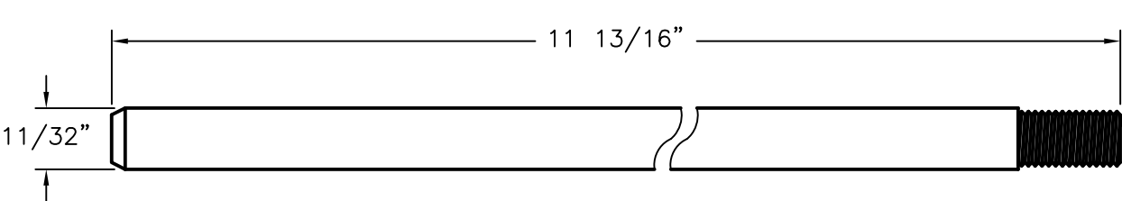
FLUSH BOLT BAR STAINLESS STEEL
