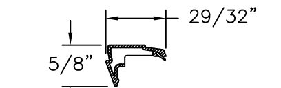
1" GLAZING BEAD EXTRUDED RIGID PVC .039" THICK
