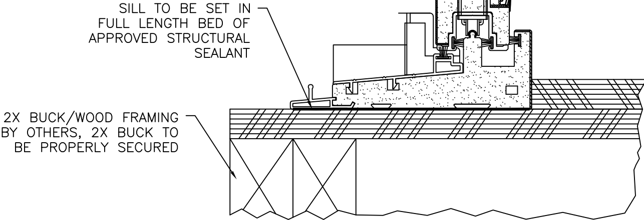
VERTICAL CROSS SECTION 2X BUCK/WOOD FRAMING
