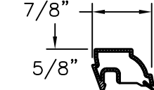
43/64" GLAZING BEAD EXTRUDED RIGID PVC
