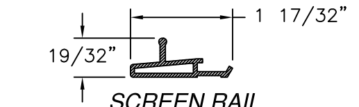
SCREEN RAIL EXTRUDED ALUMINUM 6063-T6 .059" THICK
