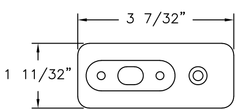
BOLT STILE END-COVER RIGID PVC
