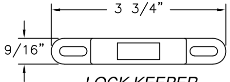
LOCK KEEPER STAINLESS STEEL
