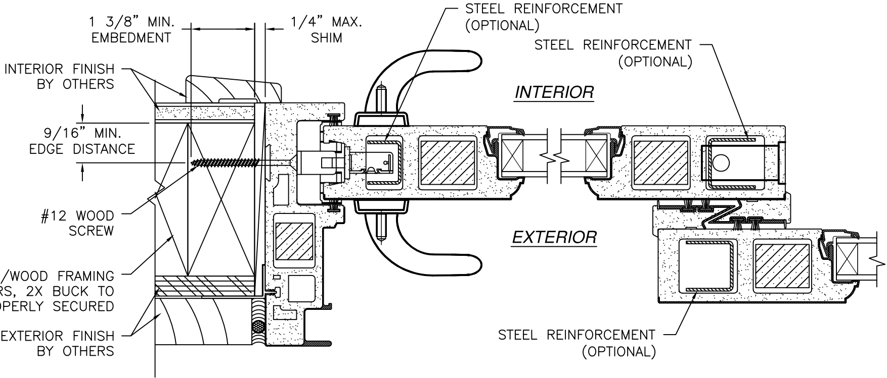
HORIZONTAL CROSS SECTION 2X BUCK/WOOD FRAMING
