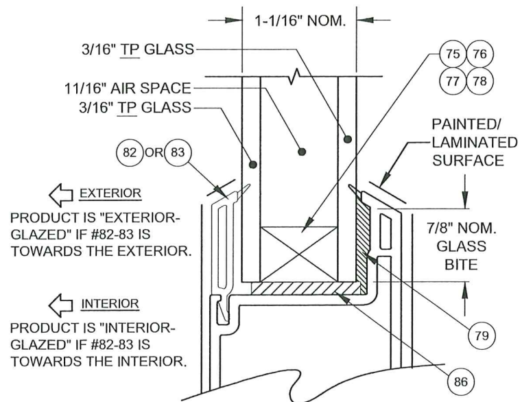
GLASS DETAIL
