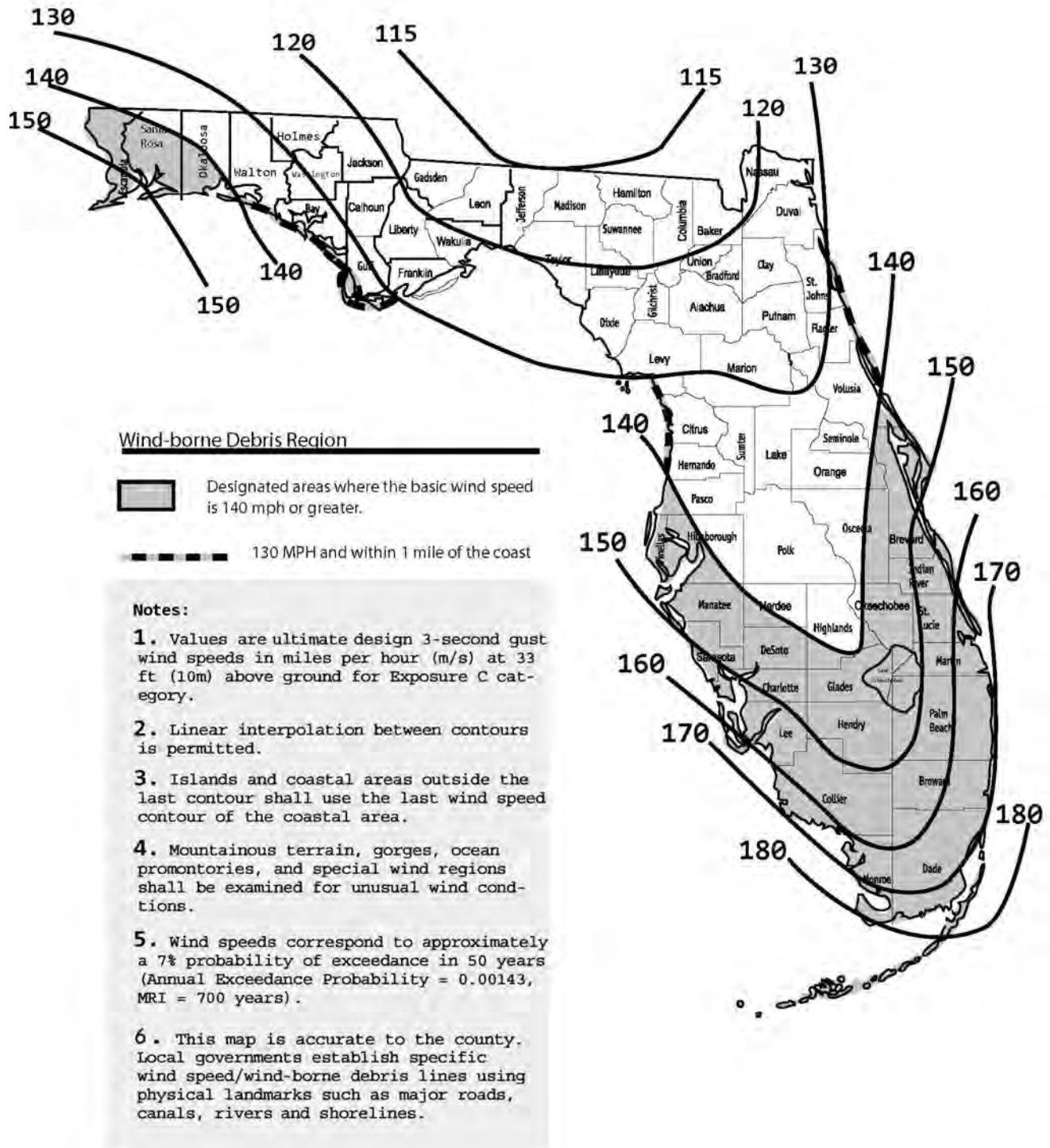
FIGURE R301.2(4) ULTIMATE DESIGN WIND SPEEDS V_{ult}
