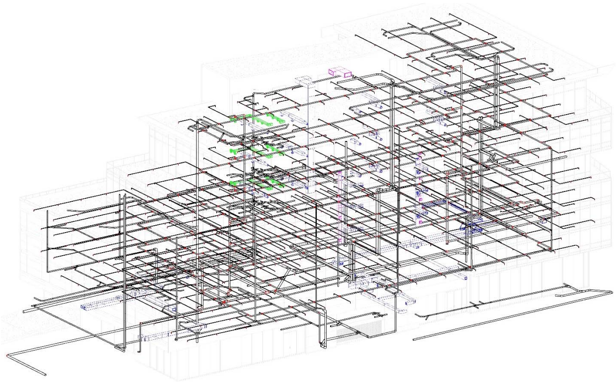
Figure A-2. 3D Model of Small Office Building
