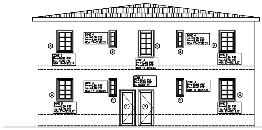
LEFT ELEVATION
