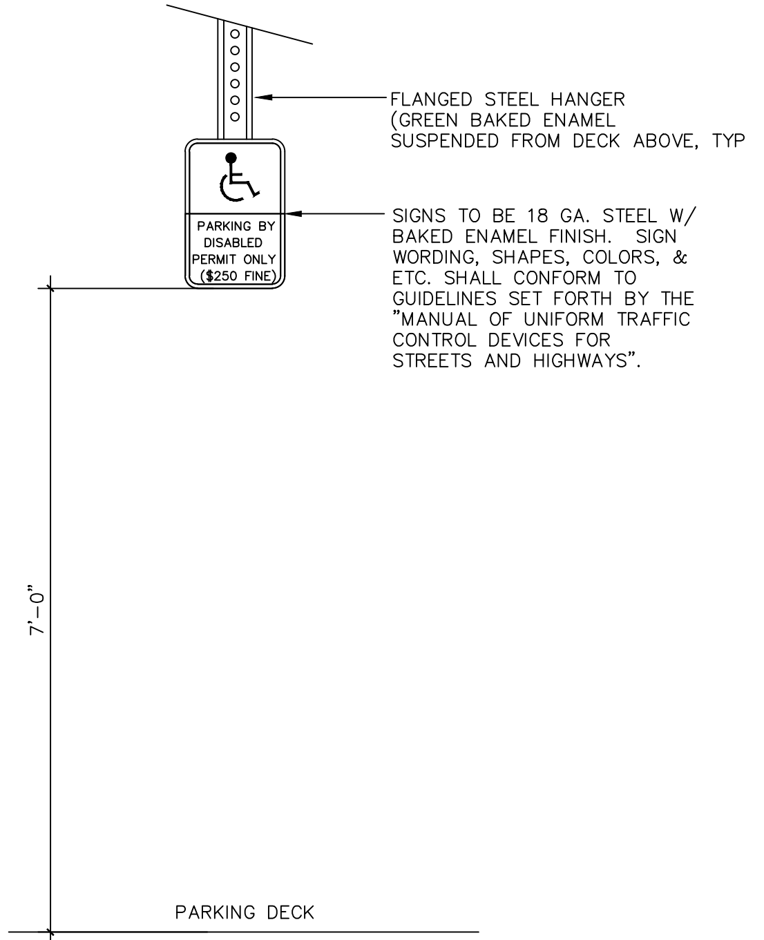
4 H/C SIGN MOUNTING HEIGHT NOT TO SCALE
