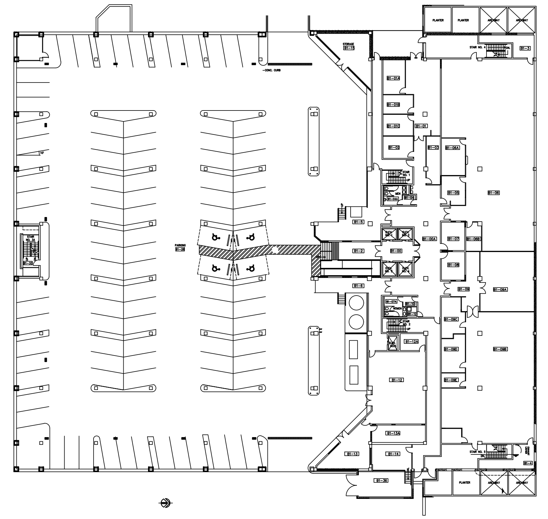
1 PARKING DECK LEVEL 1 SCALE 1/32"=1'-0"
