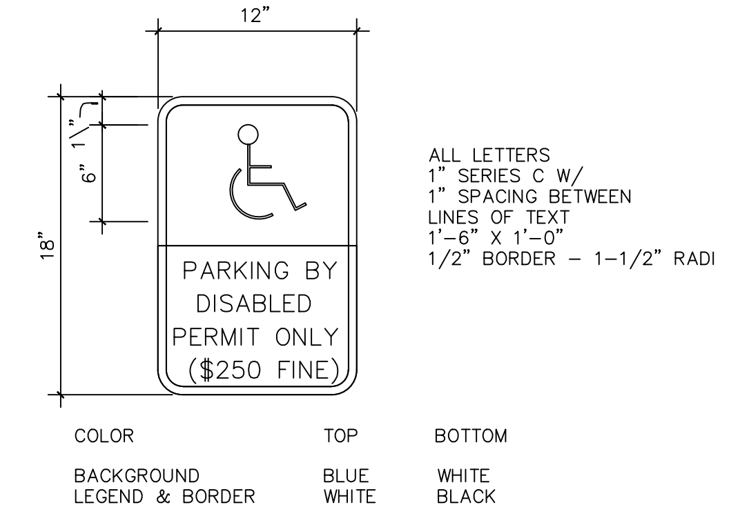
3 H/C PARKING SIGN NOT TO SCALE
