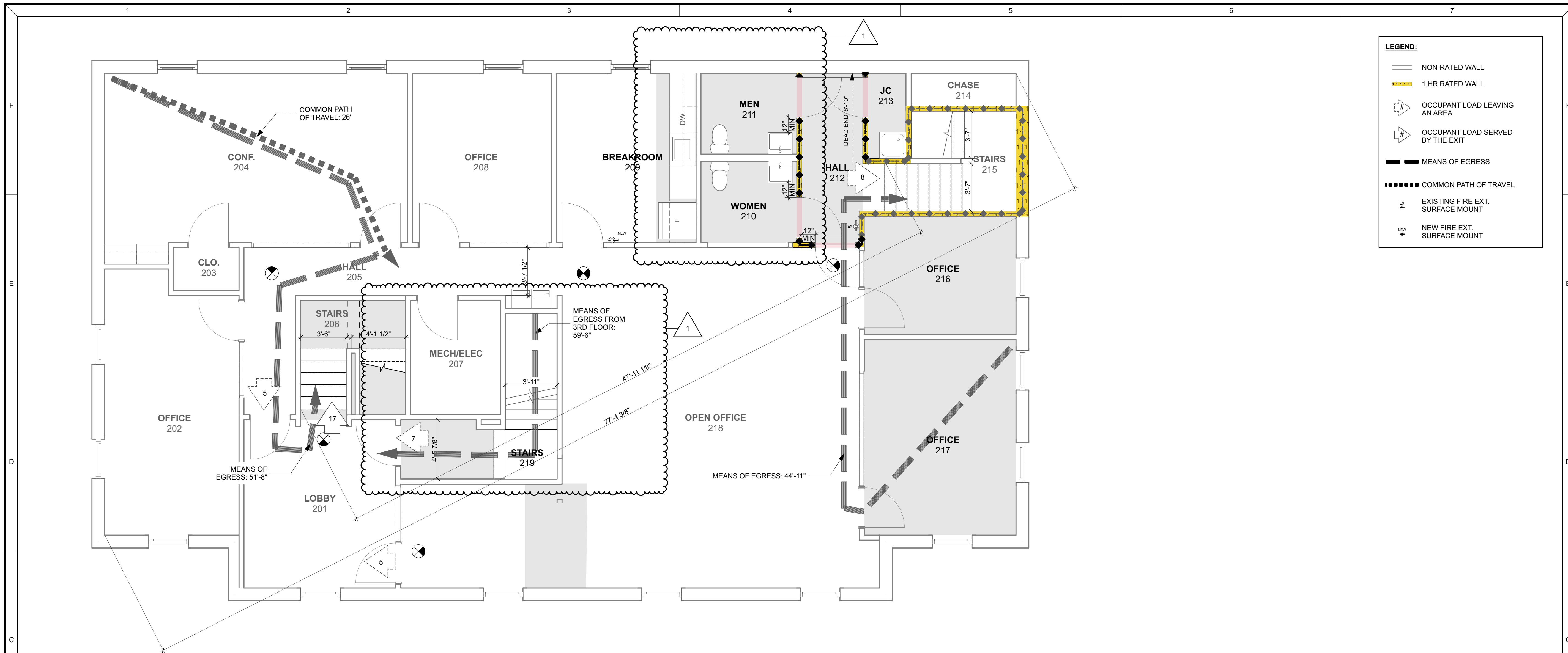
C1 SECOND FLOOR SCALE: 1/4" = 1'-0"
