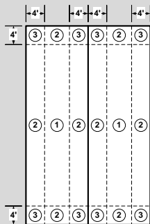
Gable Roofs 10^\circ < \theta \leq 45^\circ
