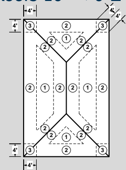
Hip Roofs 10^\circ < \theta \leq 30^\circ
