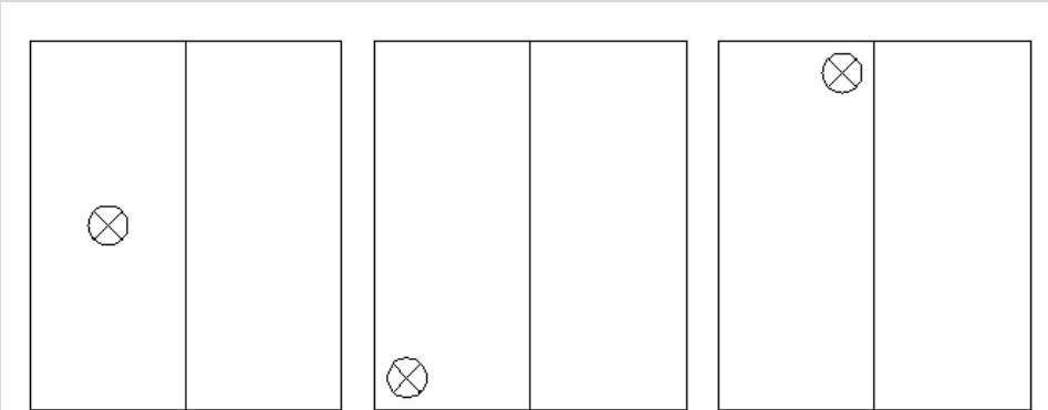
Figure 1. ASTM E1886/1996 Large Missile Impacts
