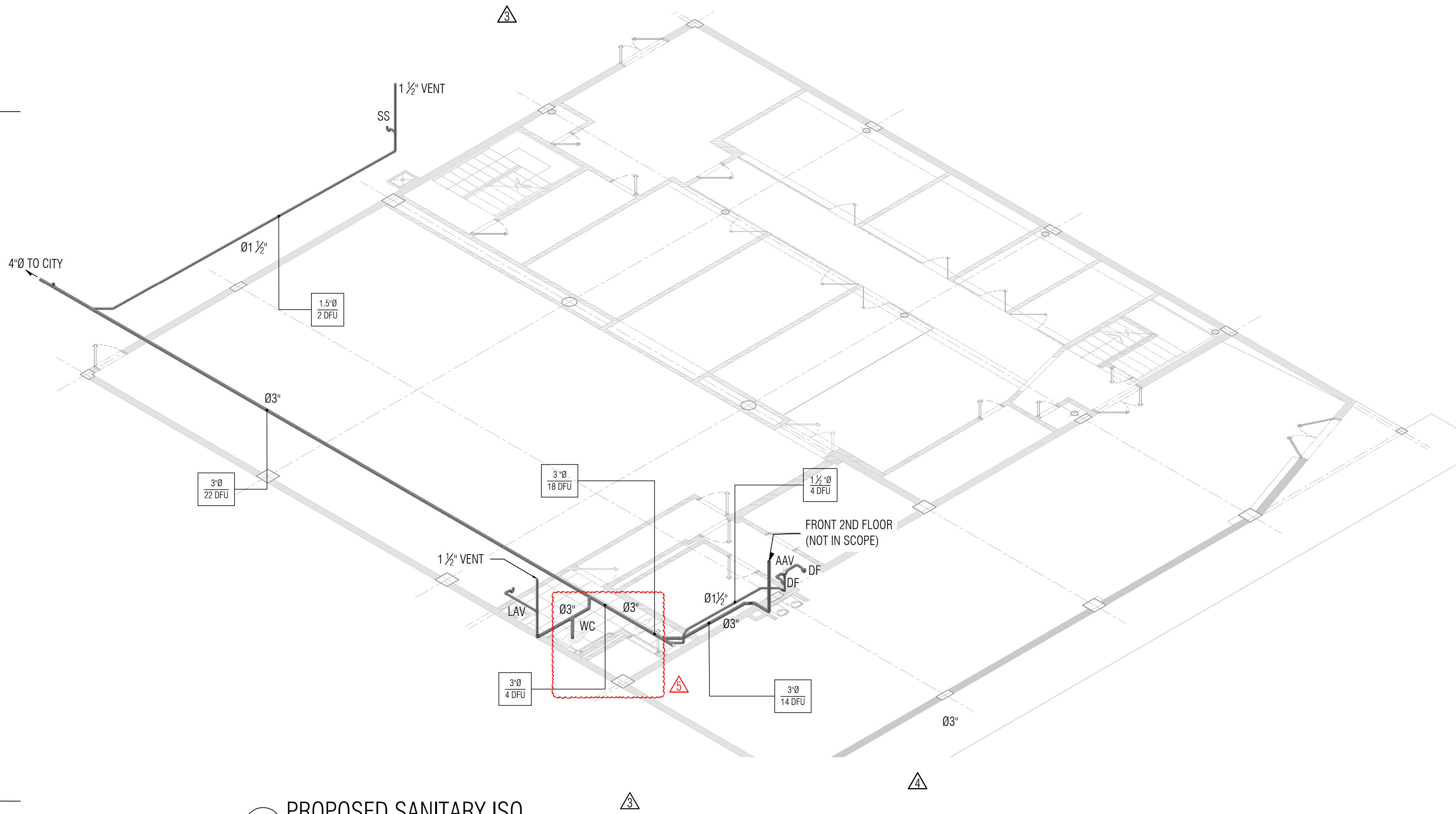
2 PROPOSED SANITARY ISO N.T.S.
