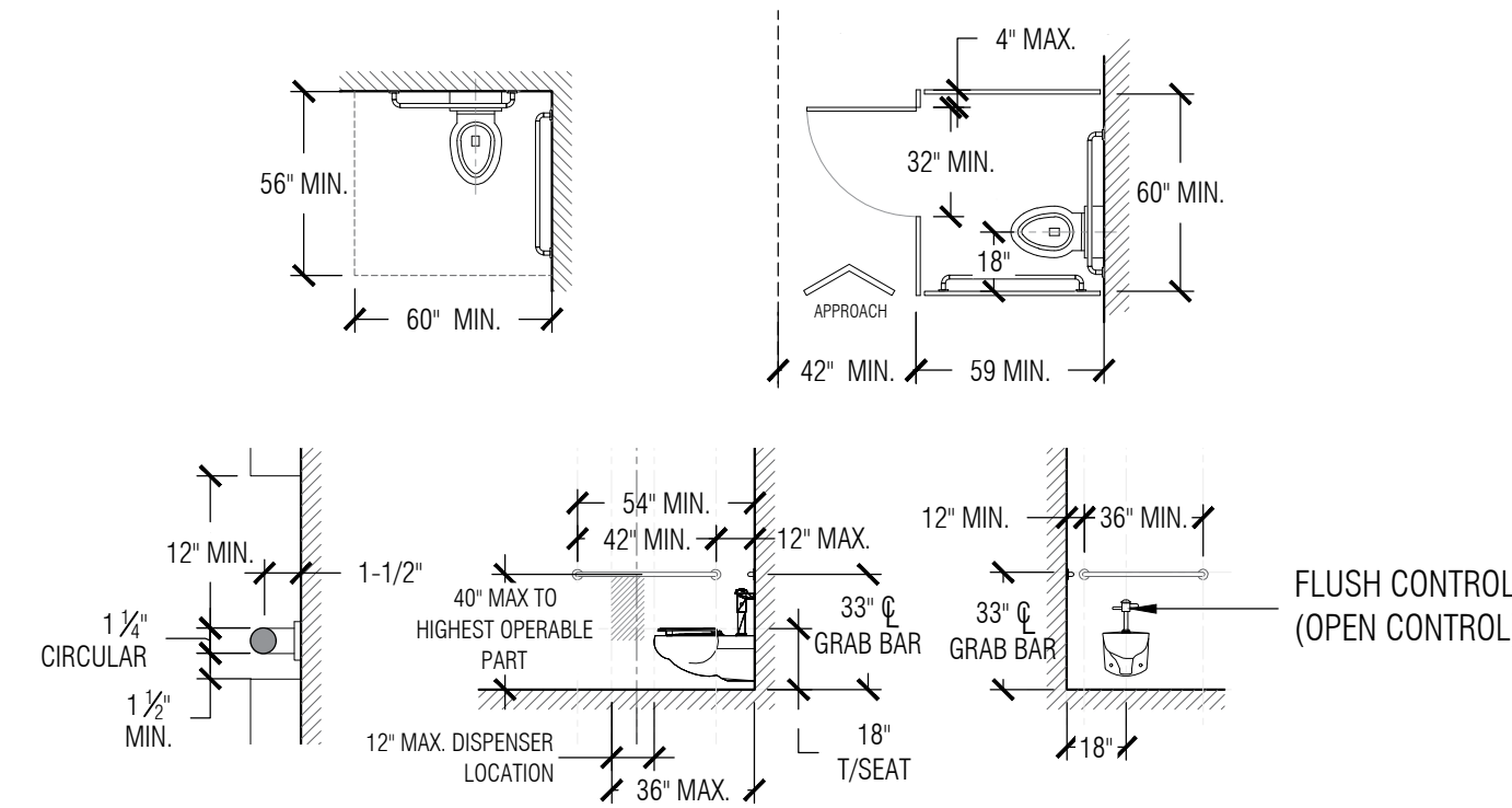
B TOILET ROOM CLEARANCES & MOUNTING HEIGHTS N.T.S.
