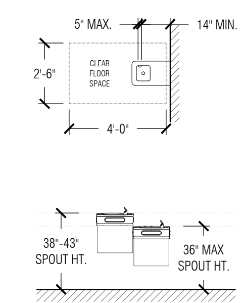
C DRINKING FOUNTAIN SPOUT LOCATION N.T.S.
