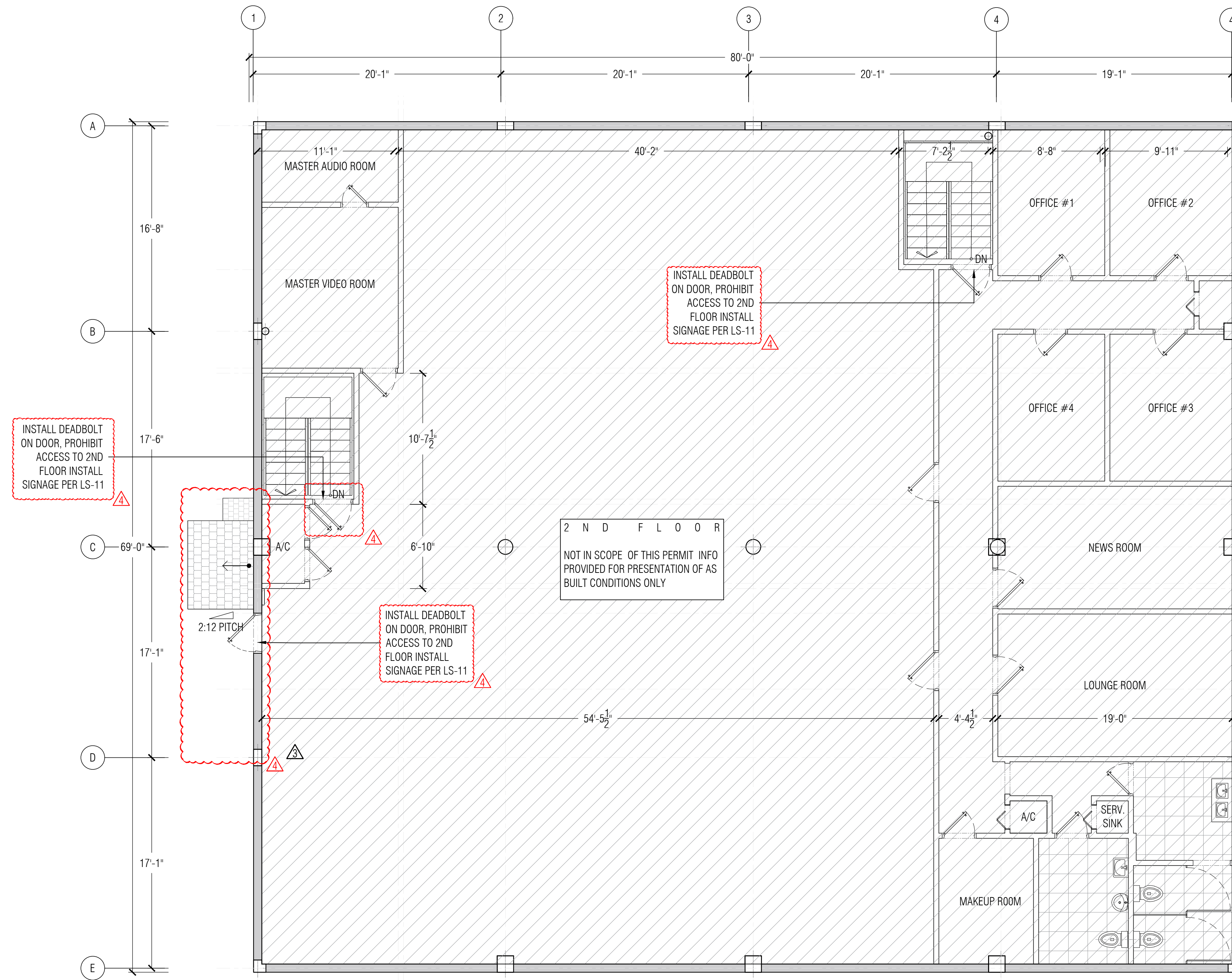
1 2ND FLOOR PLAN NOT IN SCOPE SCALE: 1/4" = 1'-0"
