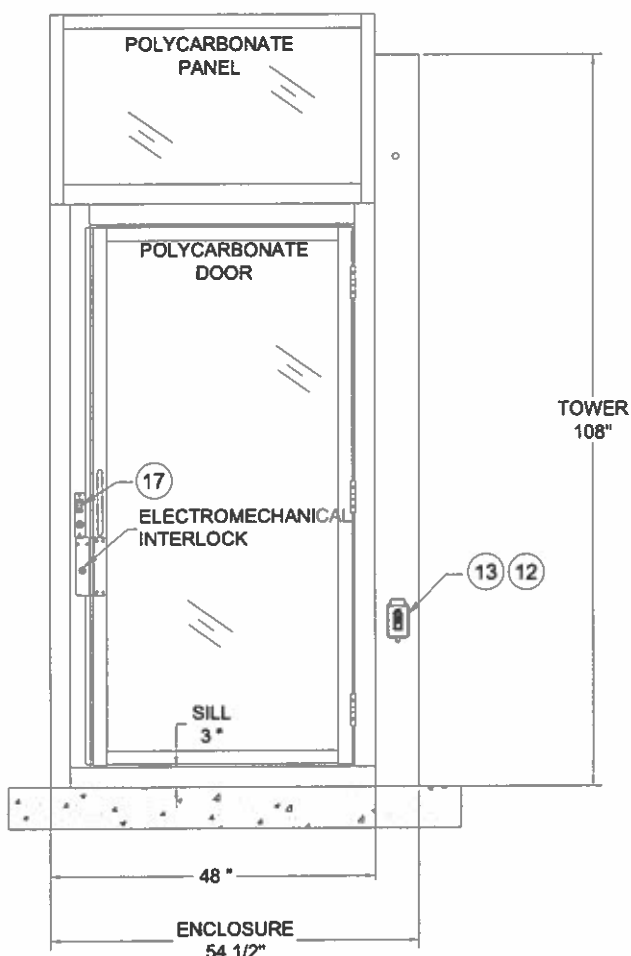
4 DETAIL A LEVEL 1
