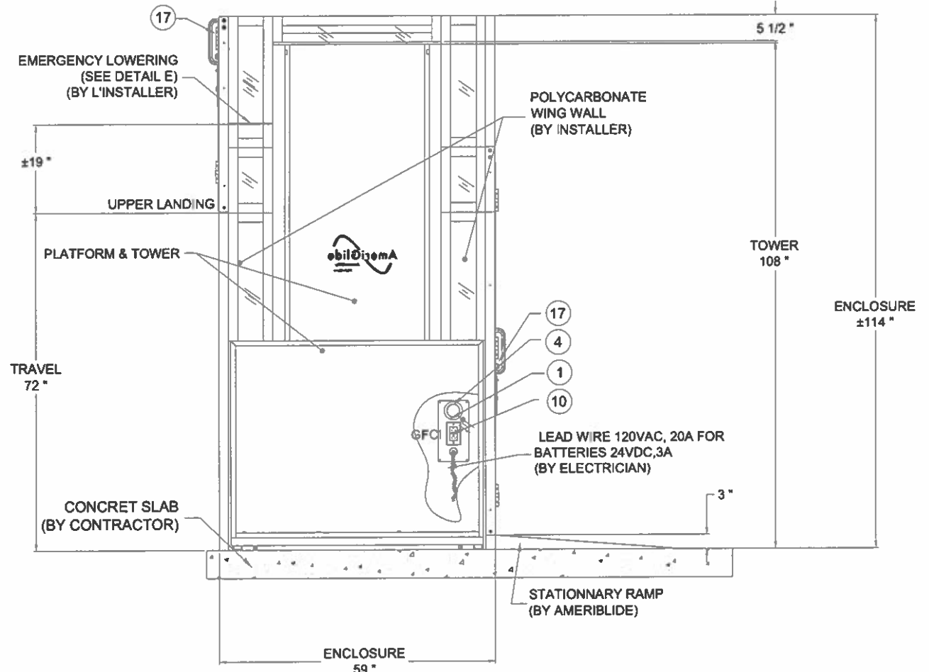
7 DETAIL D
