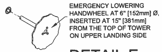
8 DETAIL E
