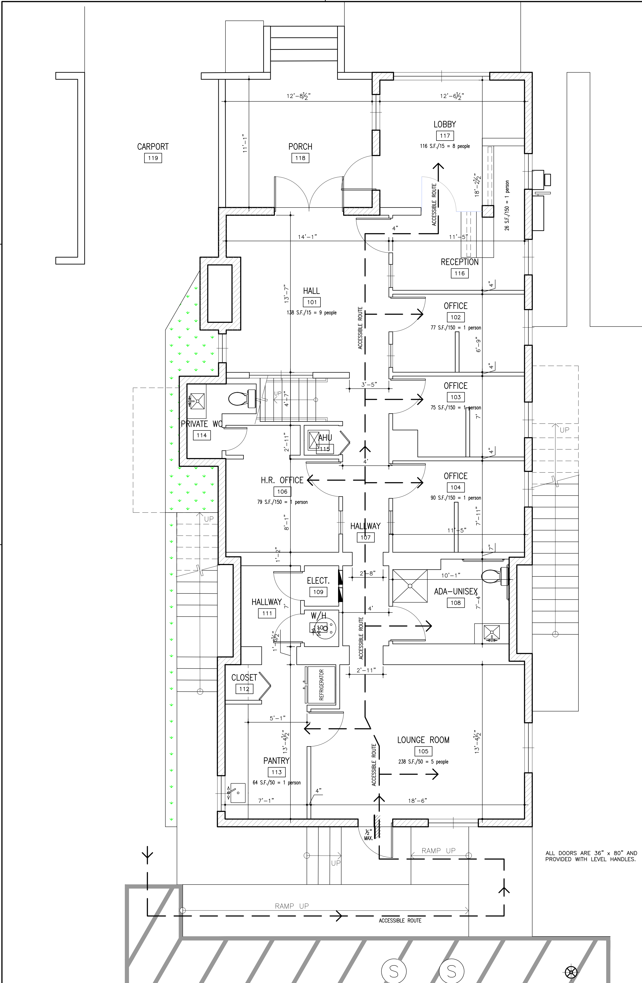
EXISTING FIRST FLOOR PLAN FOR INFORMATION ONLY SCALE: \frac{1}{4}" = 1'-0" .
