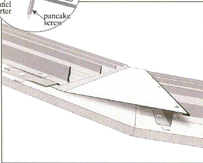
Fig. 22 Transition flashing combines the attachment techniques of valleys (top of page) with that used with ridge caps (p. 10). Notice the panel set-back that allows proper watershed from the upper panels onto the lower. The less the difference in pitch, as well as the flatter the roof, the greater the amount of set-back, and the more need for a longer "a" side on the transition flashing. The need is magnified even more for the higher-ribbed Gulf Seam panel.
