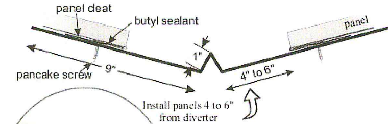
Fig. 21 Lap detail for panel cleat on transition flashing or valley.
