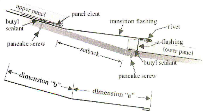
Fig. 22 Transition flashing combines the attachment techniques of valleys (top of page) with that used with ridge caps (p. 10). Notice the panel set-back that allows proper watershed from the upper panels onto the lower. The less the difference in pitch, as well as the flatter the roof, the greater the amount of set-back, and the more need for a longer "a" side on the transition flashing. The need is magnified even more for the higher-ribbed Gulf Seam panel.
