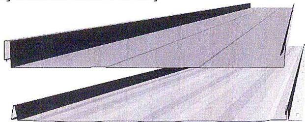
Fig. 2 The Secure-Seam panel (top) features 1 \frac{3}{4} " ribs and mounts with special clips; the 1" high Perma-Loc "nail-strip" panel (bottom) is our most popular standing seam panel. The "rib" profile is shown on the upper panel, the "striation" profile on the lower.
