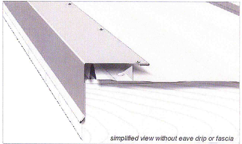
Fig. 17 Standard gable trim (EF-7) attaches to the z-flashing with rivets and to the fly rafter with either eave cleats (hidden fastener system) or exposed screws. The step rake option is shown below.
