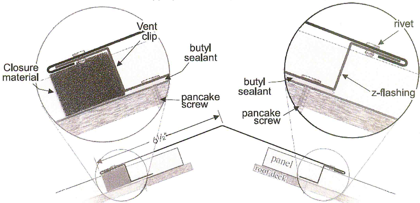
Fig. 12 Ridge caps can be installed as vented (using vent clips and vent material) or sealed (using Z-flashings), as shown also in Fig. 13
