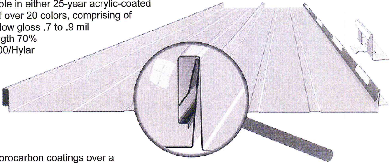
Fig. 4 Secure-Seam panels showing lap details and placement of UL-90 clips.
