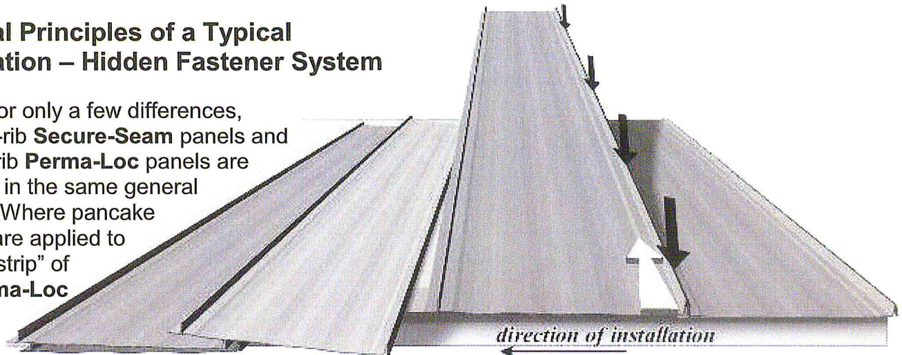
Fig. 8 Each Panel should be installed over the extended eave drip, pressed down and attached with the appropriate fasteners, and eave hems finished before installing the next panel.
