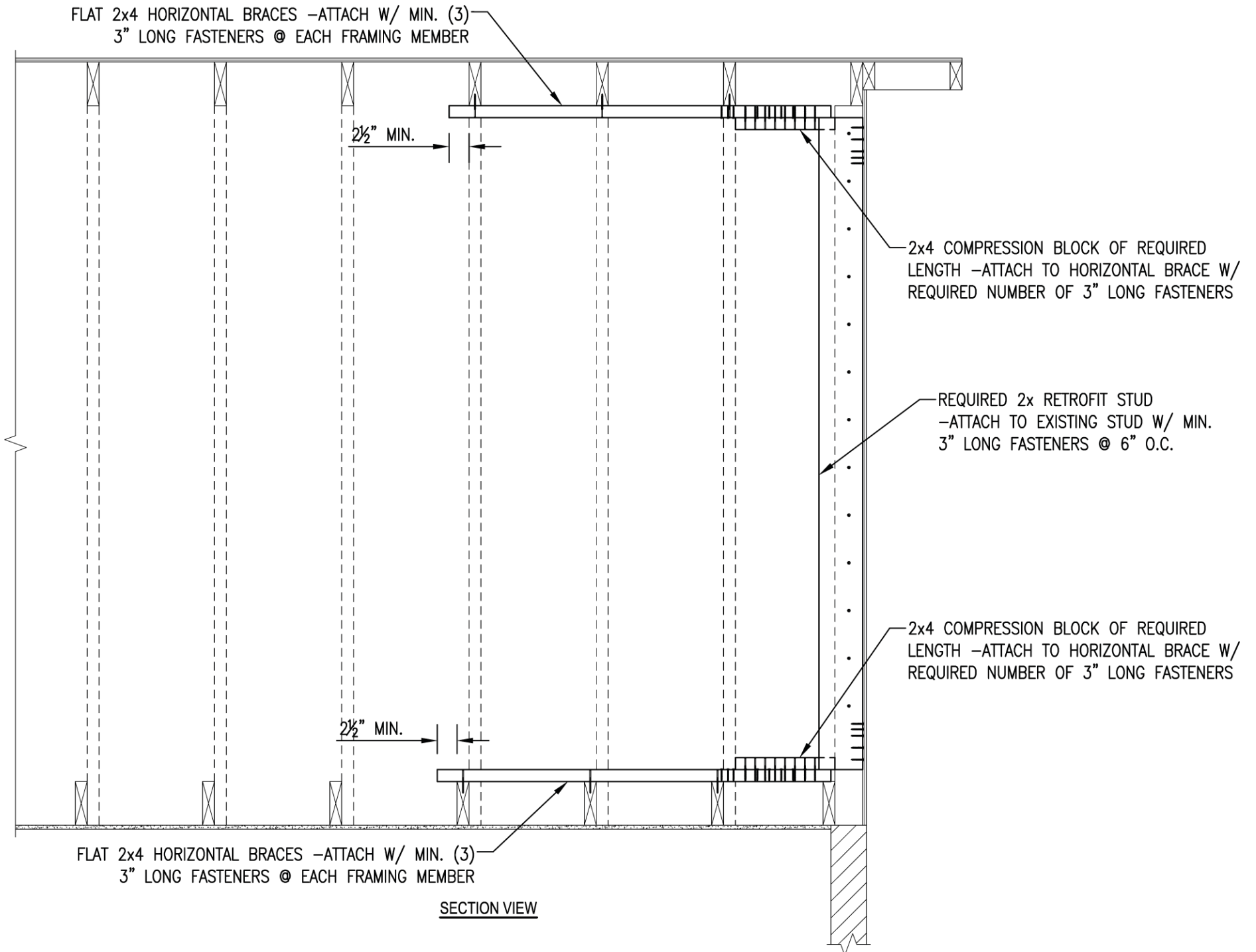
FIGURE A104.2.6 SECTION VIEW OF GABLE END RETROFIT (CONVENTIONAL FRAMED)
