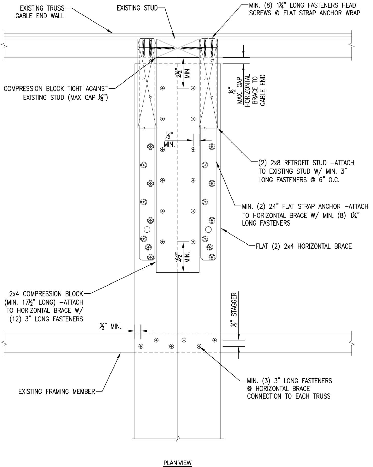
FIGURE A104.2.5 DETAILS OF STRAP & COMPRESSION BLOCK INSTALLATION - (2)2x8 RETROFIT STUD
