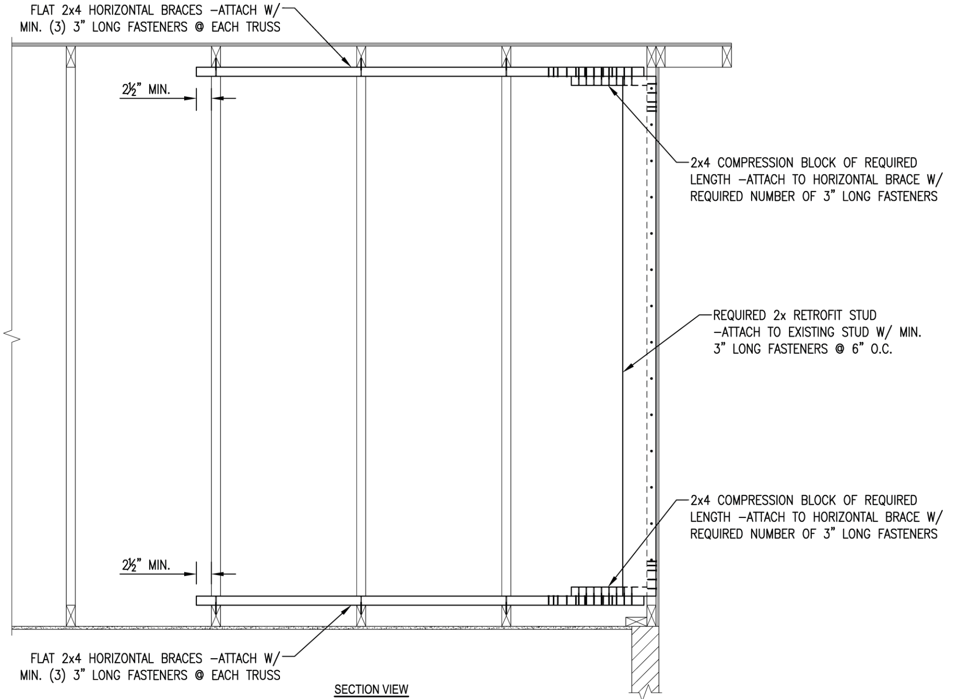
FIGURE A104.2.1 SECTION VIEW OF GABLE END RETROFIT (TRUSS WALL)
