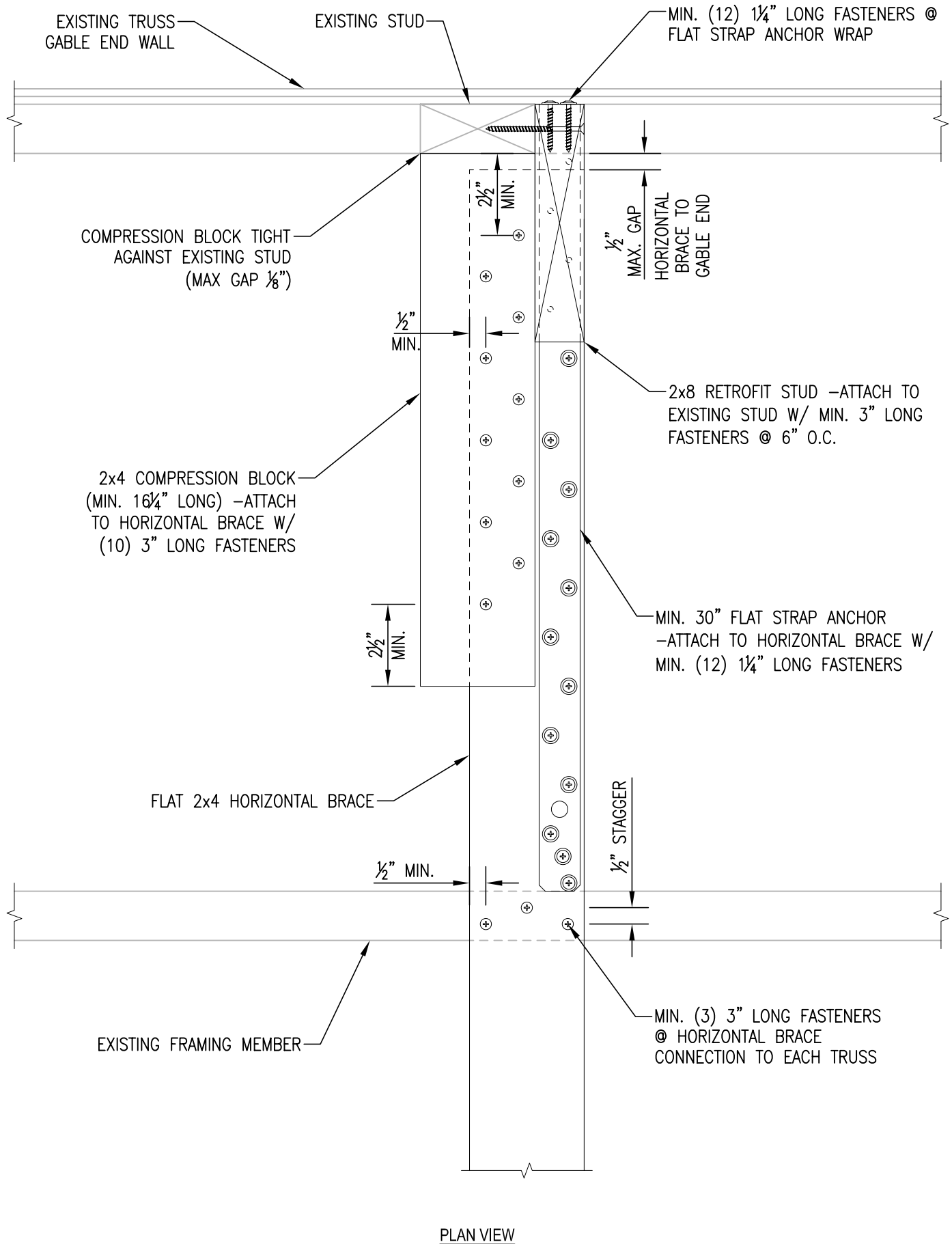
FIGURE 1504.2.4 DETAILS OF STRAP & COMPRESSION BLOCK INSTALLATION - 2x8 RETROFIT STUD
