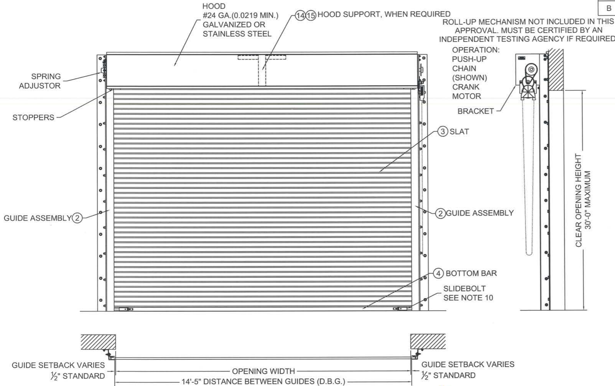
① OVERALL DOOR ASSEMBLY 1:32 SCALE
