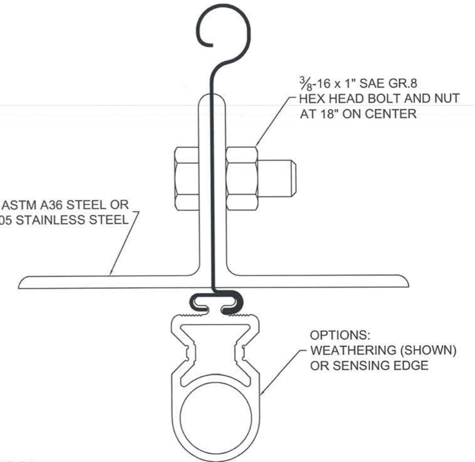
4 BOTTOM BAR DETAIL TYPICAL SECTION FULL SCALE
