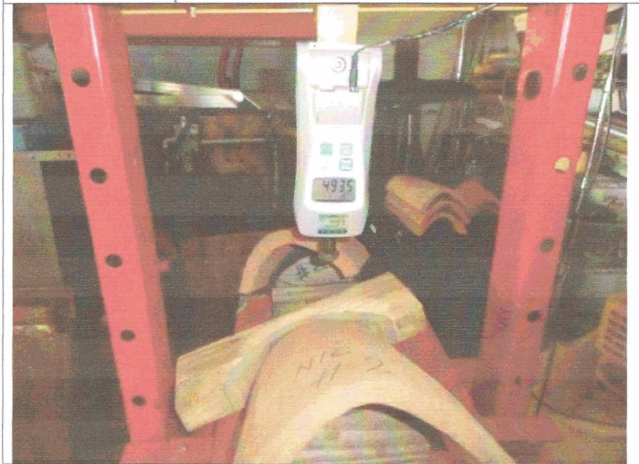
Specimen #2 Ultimate Load: 493.5 lbs.
