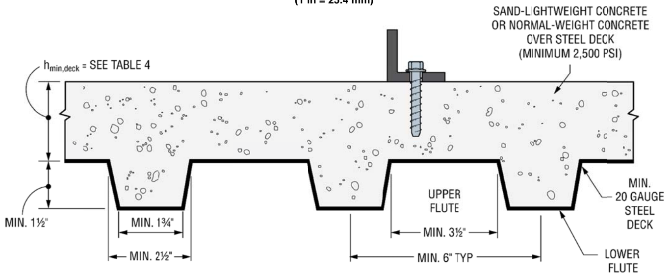
FIGURE 5—INSTALLATION OF 1/4-INCH AND 3/8-INCH SHANK DIAMETER ANCHORS IN THE TOPSIDE OF CONCRETE-FILLED PROFILE STEEL DECK FLOOR AND ROOF ASSEMBLIES (1 in = 25.4 mm)
