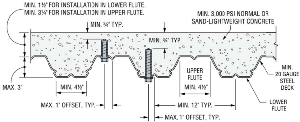
FIGURE 3—INSTALLATION OF 3/8-INCH AND 1/2-INCH SHANK DIAMETER ANCHORS IN THE SOFFIT OF CONCRETE-FILLED PROFILE STEEL DECK FLOOR AND ROOF ASSEMBLIES (1 in = 25.4 mm)
