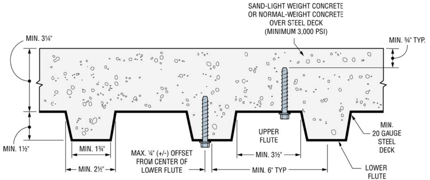
FIGURE 4—INSTALLATION OF 1/4-INCH SHANK DIAMETER ANCHOR IN THE SOFFIT OF CONCRETE-FILLED PROFILE STEEL DECK FLOOR AND ROOF ASSEMBLIES (1 in = 25.4 mm)
