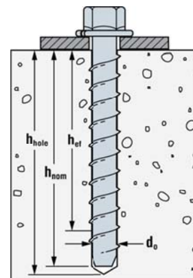
FIGURE 2—TITEN HD® SCREW ANCHOR INSTALLATION
