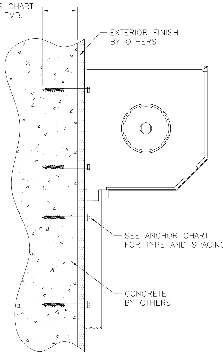
SECTION A-A CONCRETE INSTALLATION SHOWN SEE CHART SHEETS 7-9 FOR OTHER SUBSTRATES SLATS NOT SHOWN FOR CLARITY
