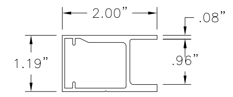
23 SPACER 6063-T5 ALUMINUM TRIM FROM SIDE RAIL
