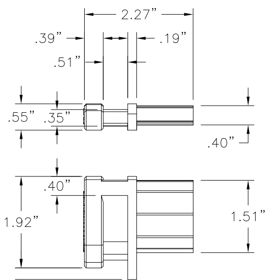
(24) END RETENTION - RIGHT NYLON
