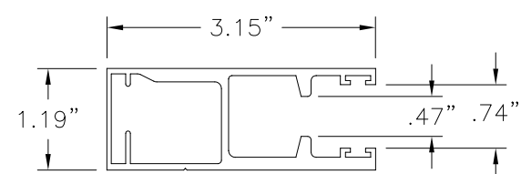
(31) SIDE RAIL FOR END RETENTION 6063-T5 ALUMINUM
