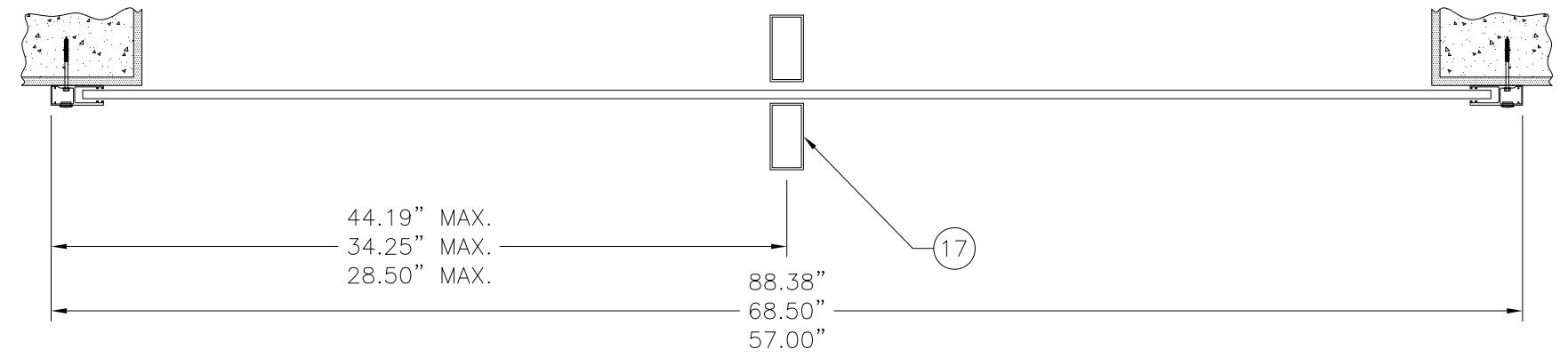
STORM BAR LOCATION FOR 88.38\", 68.50\" AND 50.78\" UNITS WITH ONE STORM BAR
