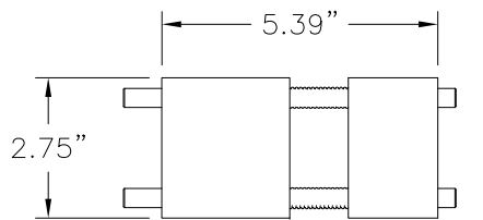
(30) 2X3 SPRING BLOCK
