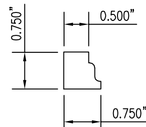
9 GLAZING BEAD Scale: 1/2 FULL SIZE
