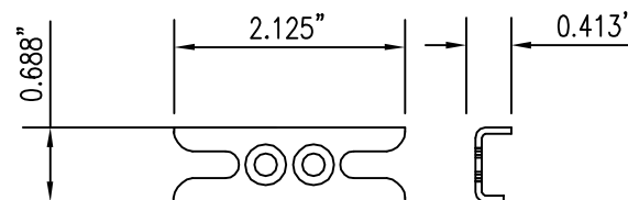
10 CAM KEEPERS Scale: 1/2 FULL SIZE
