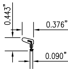
21 GASKET QEZD 320 Scale: 1/2 FULL SIZE
