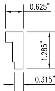
7 FIXED SASH BLOCK Scale: 1/2 FULL SIZE
