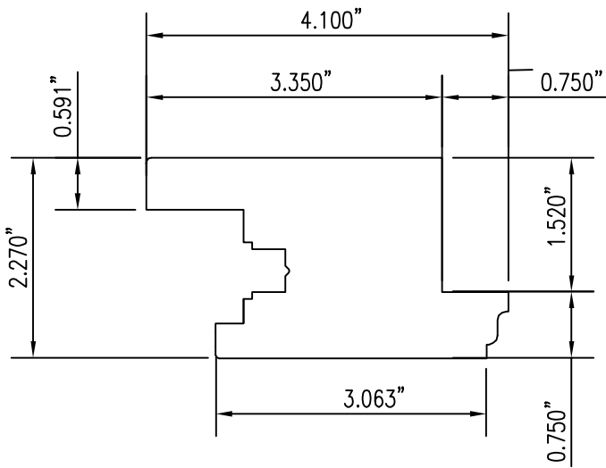
4 INACTIVE MEETING STILE Scale: 1/2 FULL SIZE
