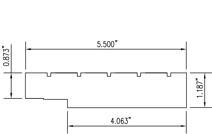
1 HEAD, SILL & SIDE JAMB Scale: 1/2 FULL SIZE
