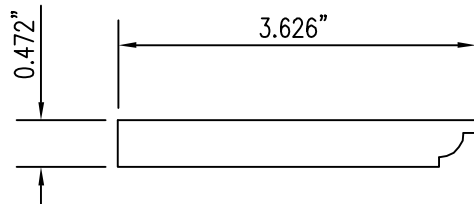
5 INTERIOR TRIM/STOP Scale: 1/2 FULL SIZE
