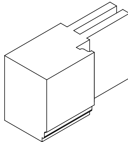
A SASH - 3 FINGER JONT
