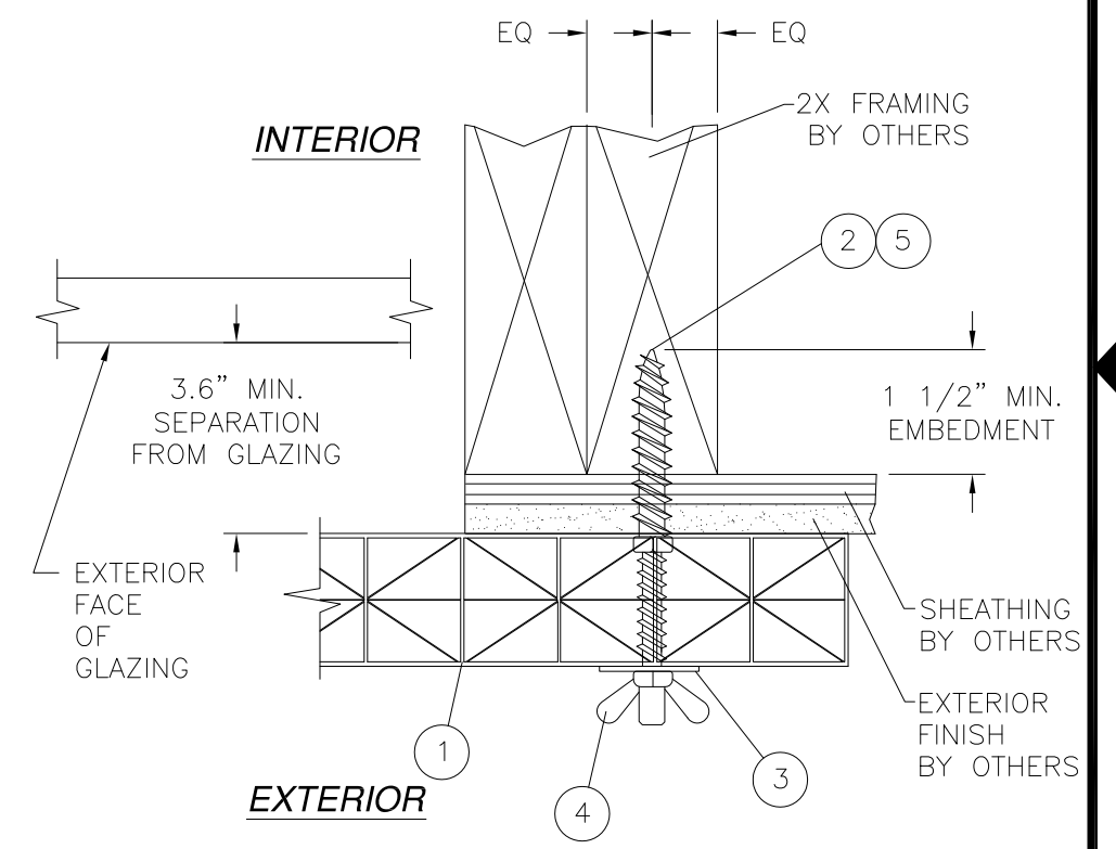
B 2 SECTION WOOD FRAMING INSTALLATION
