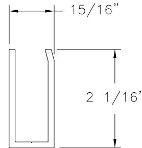
⑥ U-CHANNEL ALUMINUM 6063-T5 1/8" THICK
