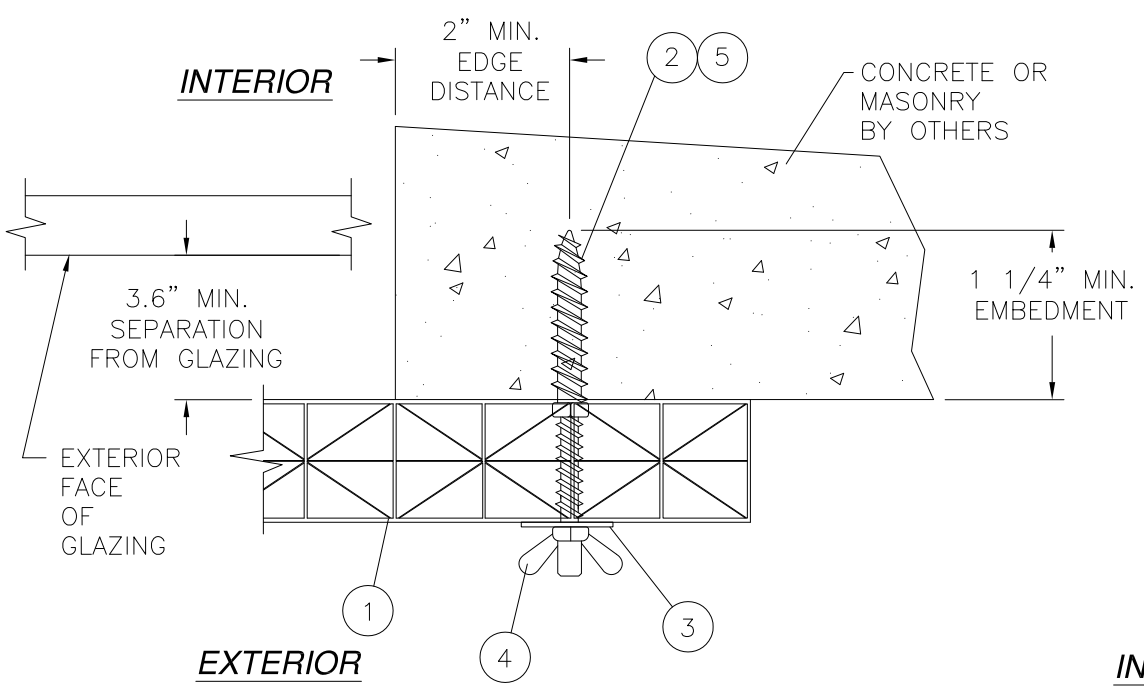
B 2 SECTION CONCRETE OR MASONRY INSTALLATION
