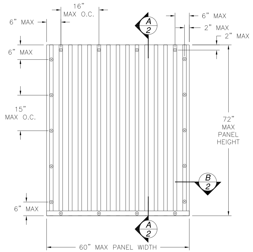
5/8" PANEL EXTERIOR VIEW
