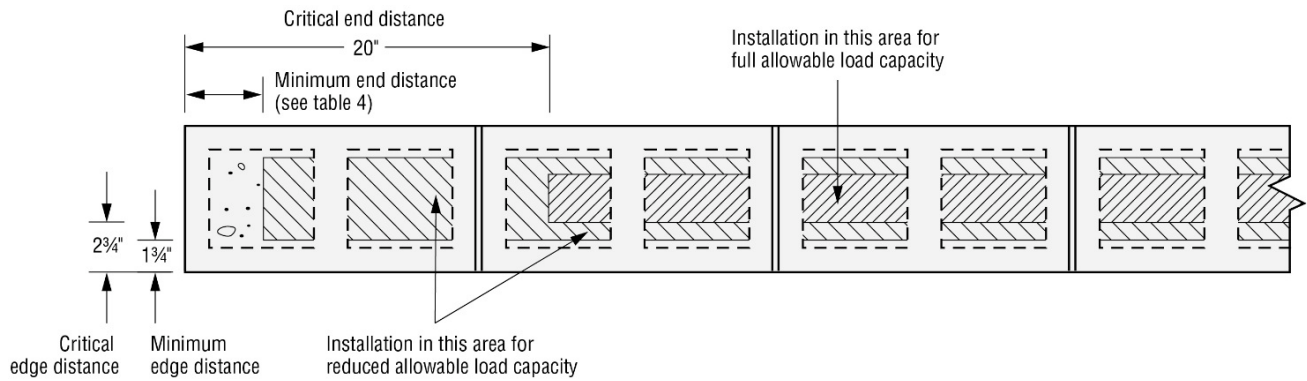
FIGURE 3A – 1/2 INCH AND 5/8 INCH DIAMETER THREADED ROD ALLOWABLE ANCHOR LOCATIONS FOR FULL AND REDUCED LOAD CAPACITY WHEN INSTALLATION IS IN THE TOP OF FULLY GROUTED CMU MASONRY WALL CONSTRUCTION
