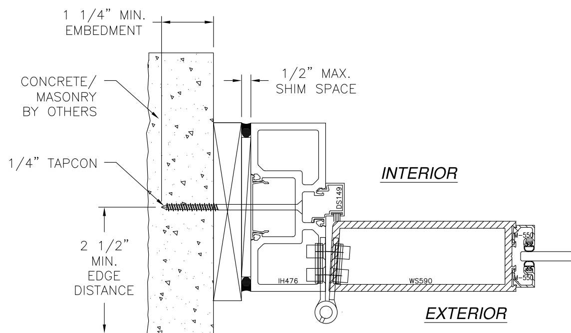
JAMB INSTALLATION DETAIL CONCRETE/MASONRY INSTALLATION
