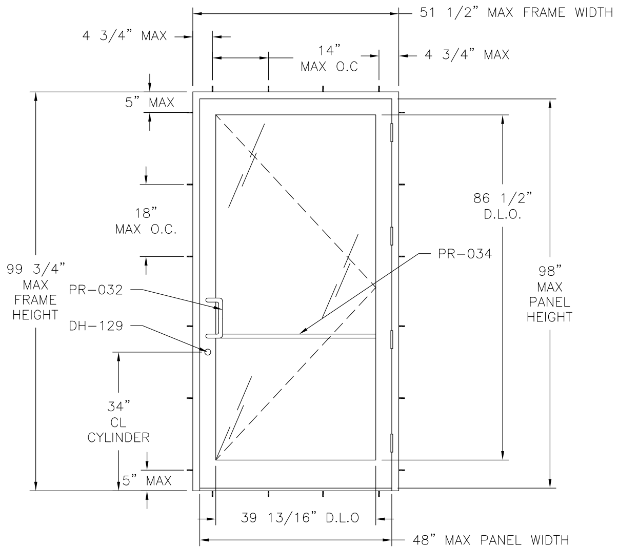
SERIES 850 SLUMINUM SINGLE DOOR EXTERIOR VIEW FRAME FLUSH INSTALLATION
