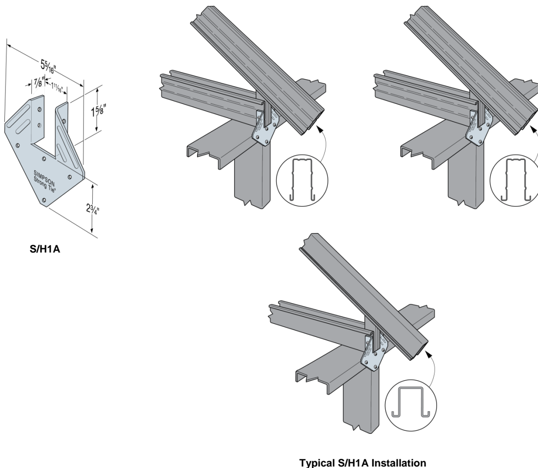
FIGURE 9 – S/H1A HURRICANE TIE
