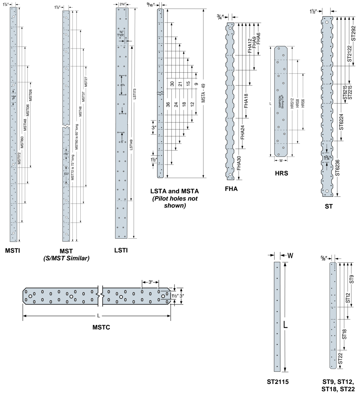
FIGURE 10 - STRAPS
