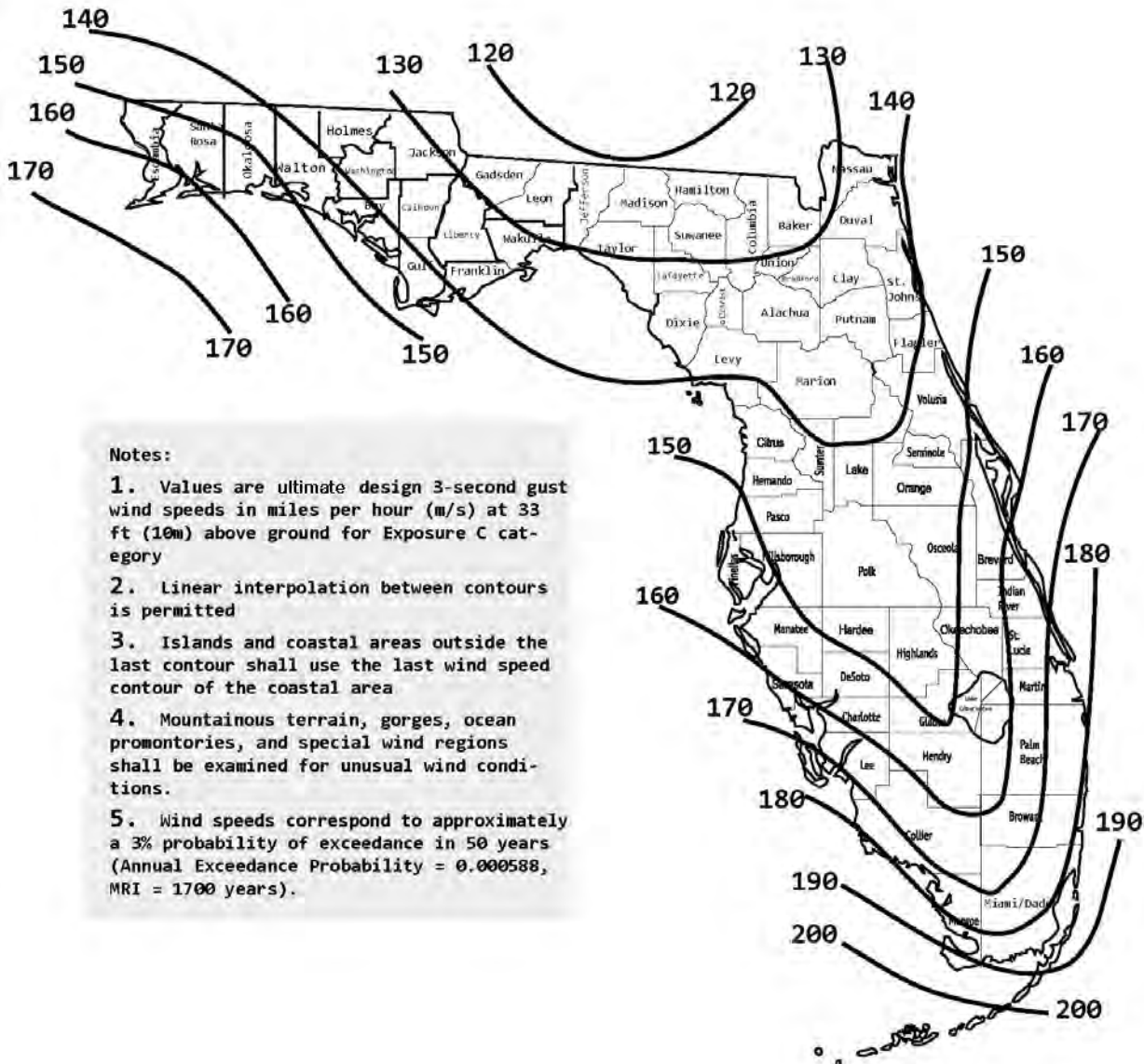
FIGURE 1609.3(2) ULTIMATE DESIGN WIND SPEEDS, V_{UL} , FOR RISK CATEGORY III AND IV BUILDINGS AND OTHER STRUCTURES
