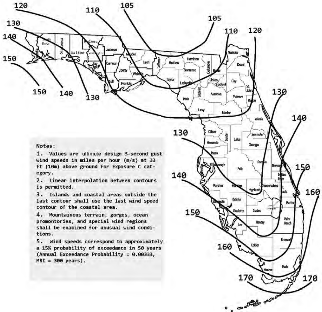
FIGURE 1609.3(3) ULTIMATE DESIGN WIND SPEEDS, V_{UL} , FOR RISK CATEGORY I BUILDINGS AND OTHER STRUCTURES
