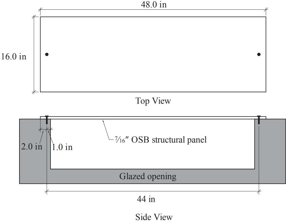
Figure 11. Panel used in experimental testing
