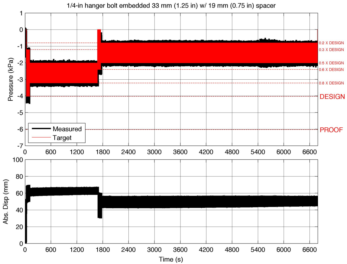
Figure 8. Cyclic pressure loading sequence derived from ASTM E1996 for Case 1 (2.00 inch embedment) for the negative pressure case
