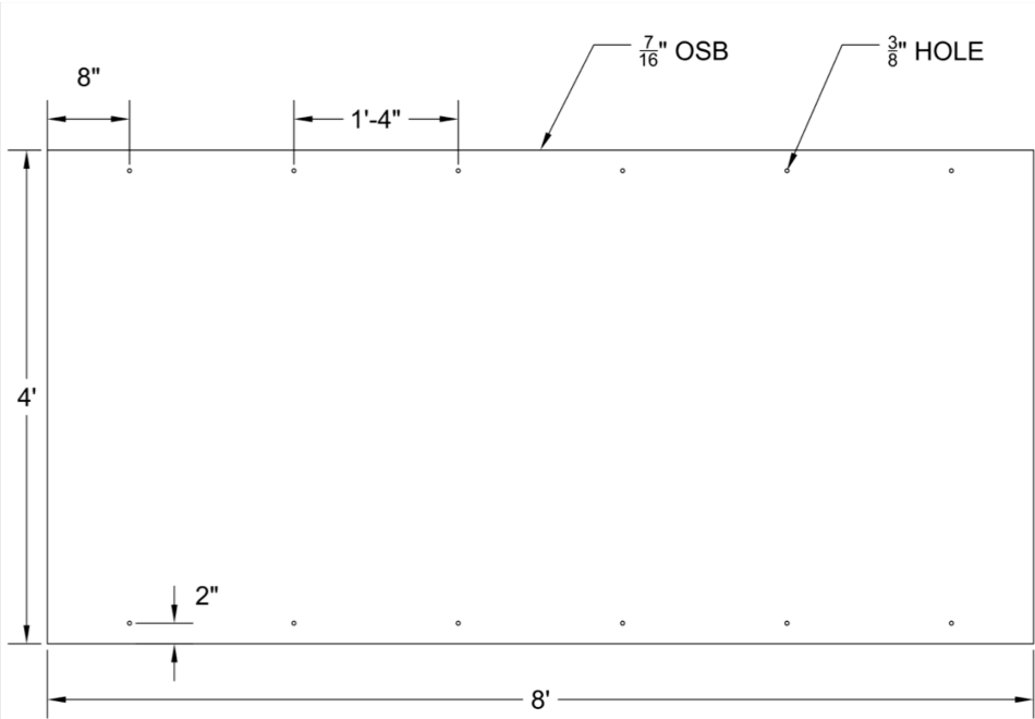
Figure 4. Shutter configuration
