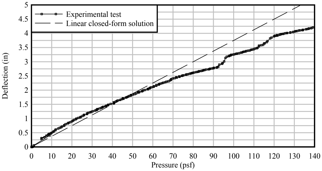
Figure 17. Validation of recommended closed form solution for deflection (load applied toward building)
