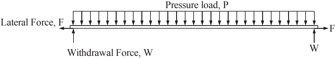
Figure 12. Free body diagram of panel undergoing beam action with catenary effects.
