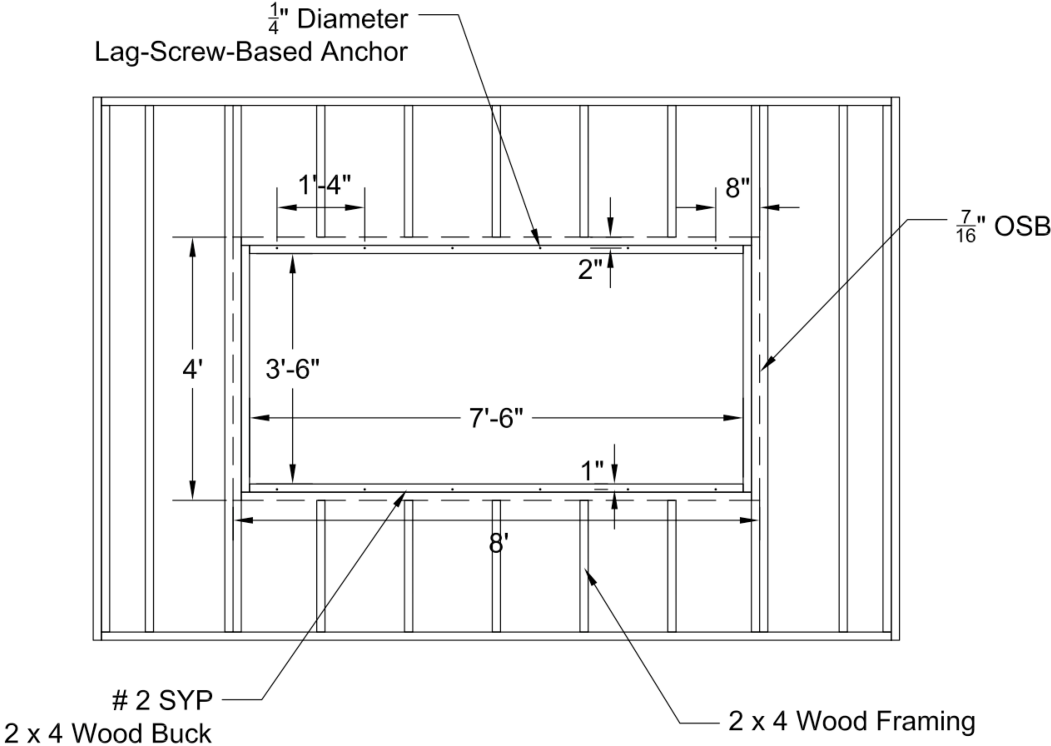
Figure 3. Wood frame wall configuration
