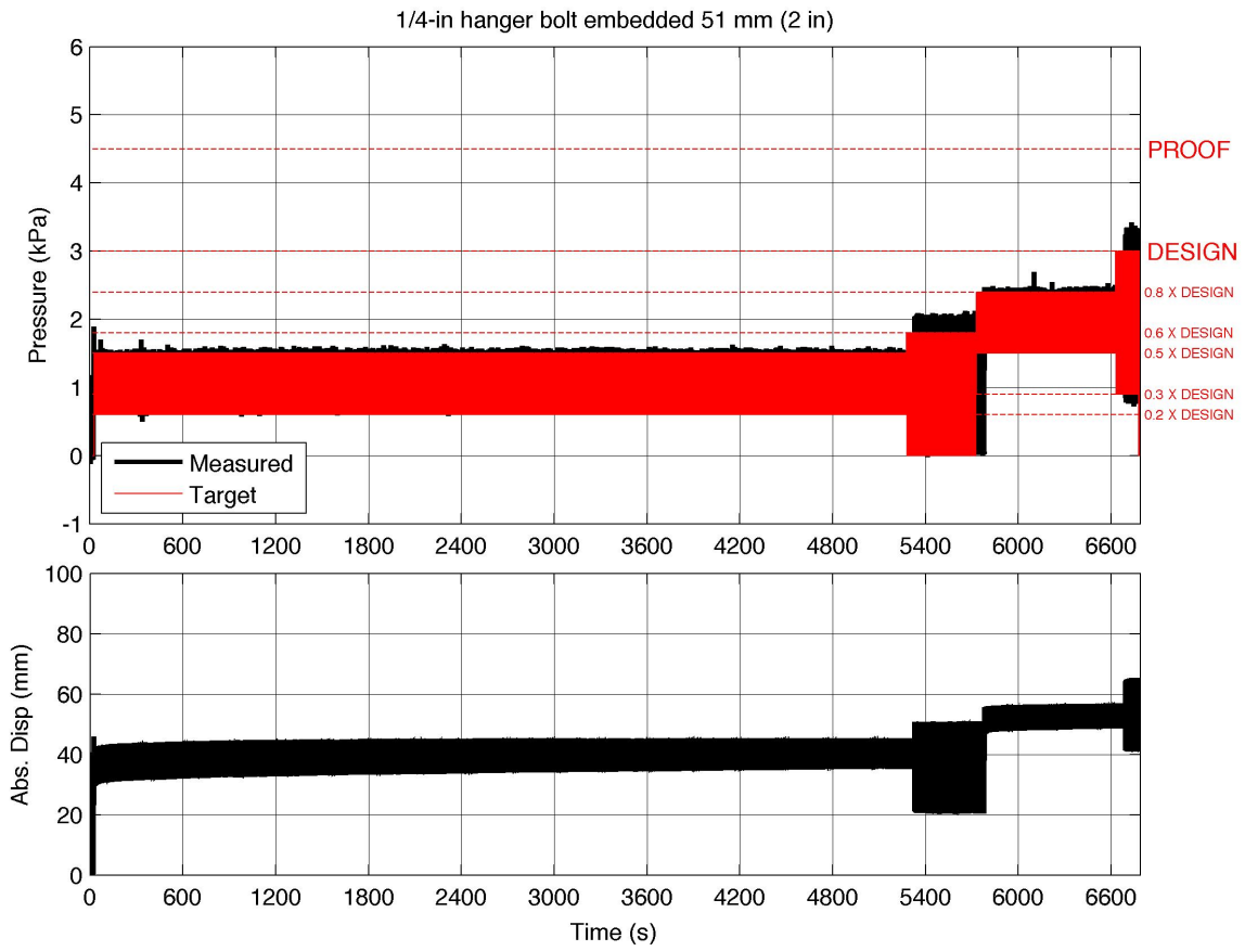
Figure 9. Cyclic pressure loading sequence derived from ASTM E1996 for Case 2 (1.25 inch embedment) for the positive pressure case
