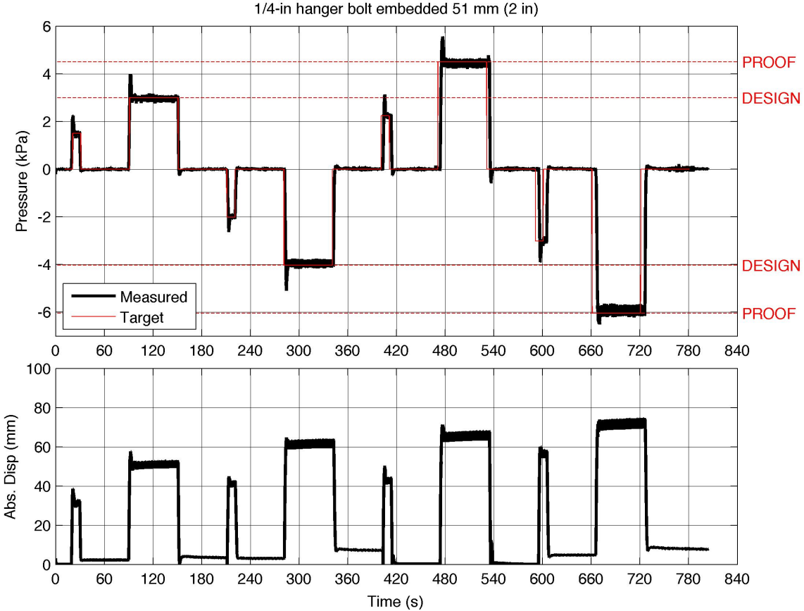
Figure 5. Static pressure loading sequence derived from ASTM E 330 for Case 1 (2.00 inch embedment)
