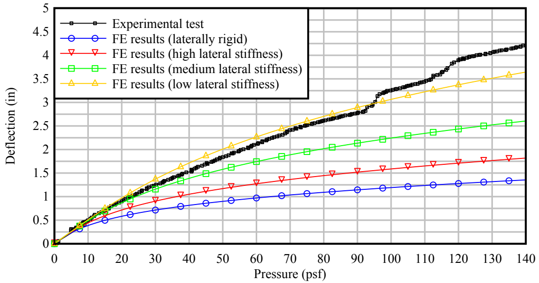
Figure 13. Comparison between experimentally-measured deflections and FEA results in the towards-the-building load direction
