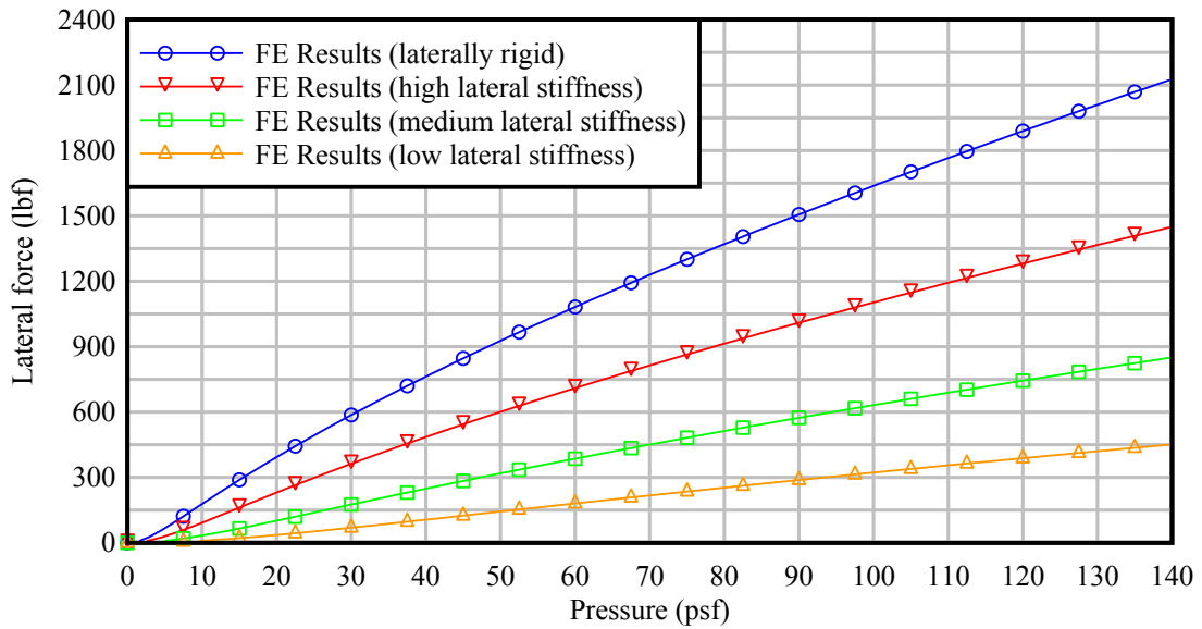
Figure 16. Comparison between FE lateral force results for different lateral stiffnesses in the away-from-the-building load direction
