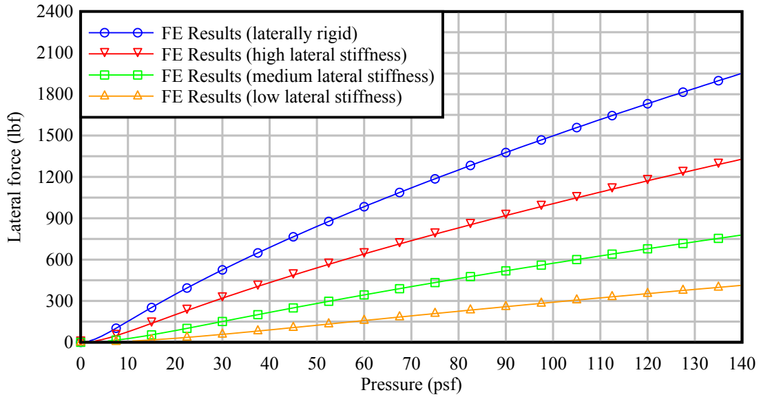
Figure 15. Comparison between FE lateral force results for different lateral stiffnesses in the toward-the-building load direction
