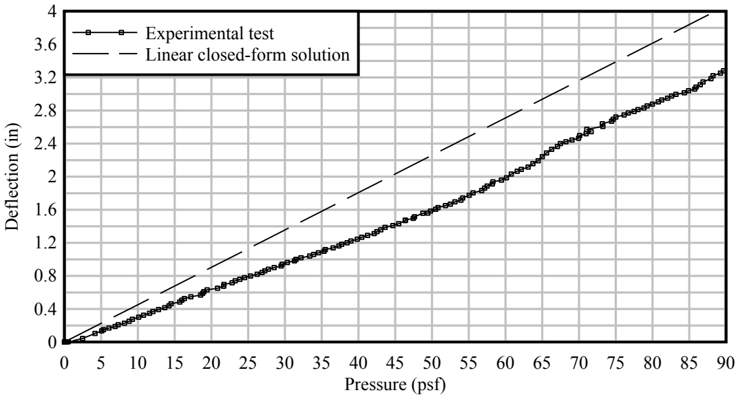
Figure 18. Validation of recommended closed form solution for deflection (load applied away from building)
