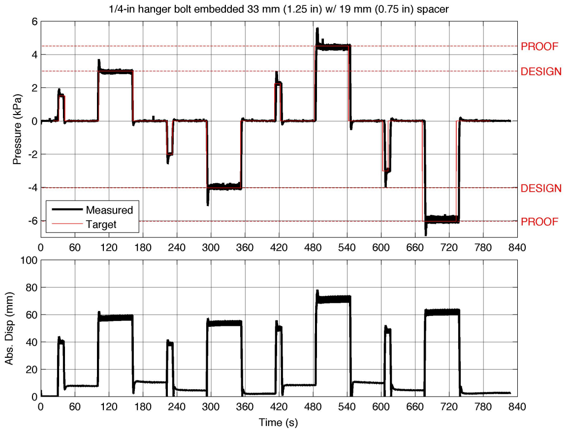
Figure 6. Static pressure loading sequence derived from ASTM E 330 for Case 2 (1.25 inch embedment)
