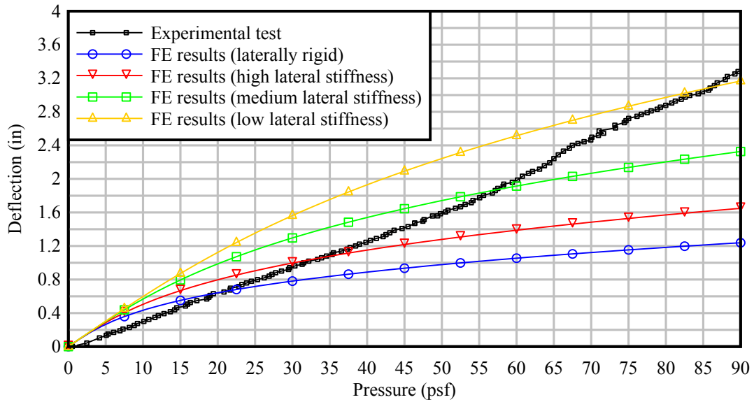
Figure 14. Comparison between experimentally-measured deflections and FEA results in the away-from-the-building load direction
