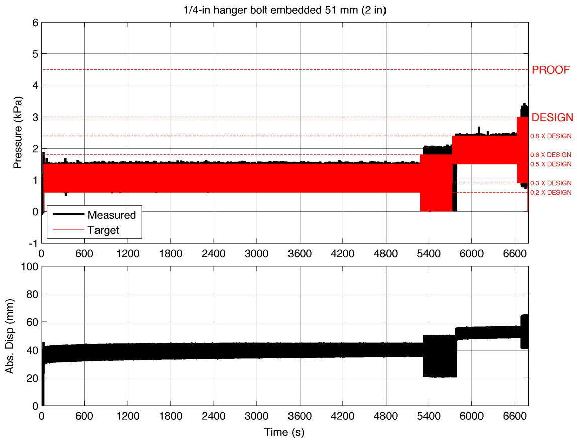
Figure 7. Cyclic pressure loading sequence derived from ASTM E1996 for Case 1 (2.00 inch embedment) for the positive pressure case
