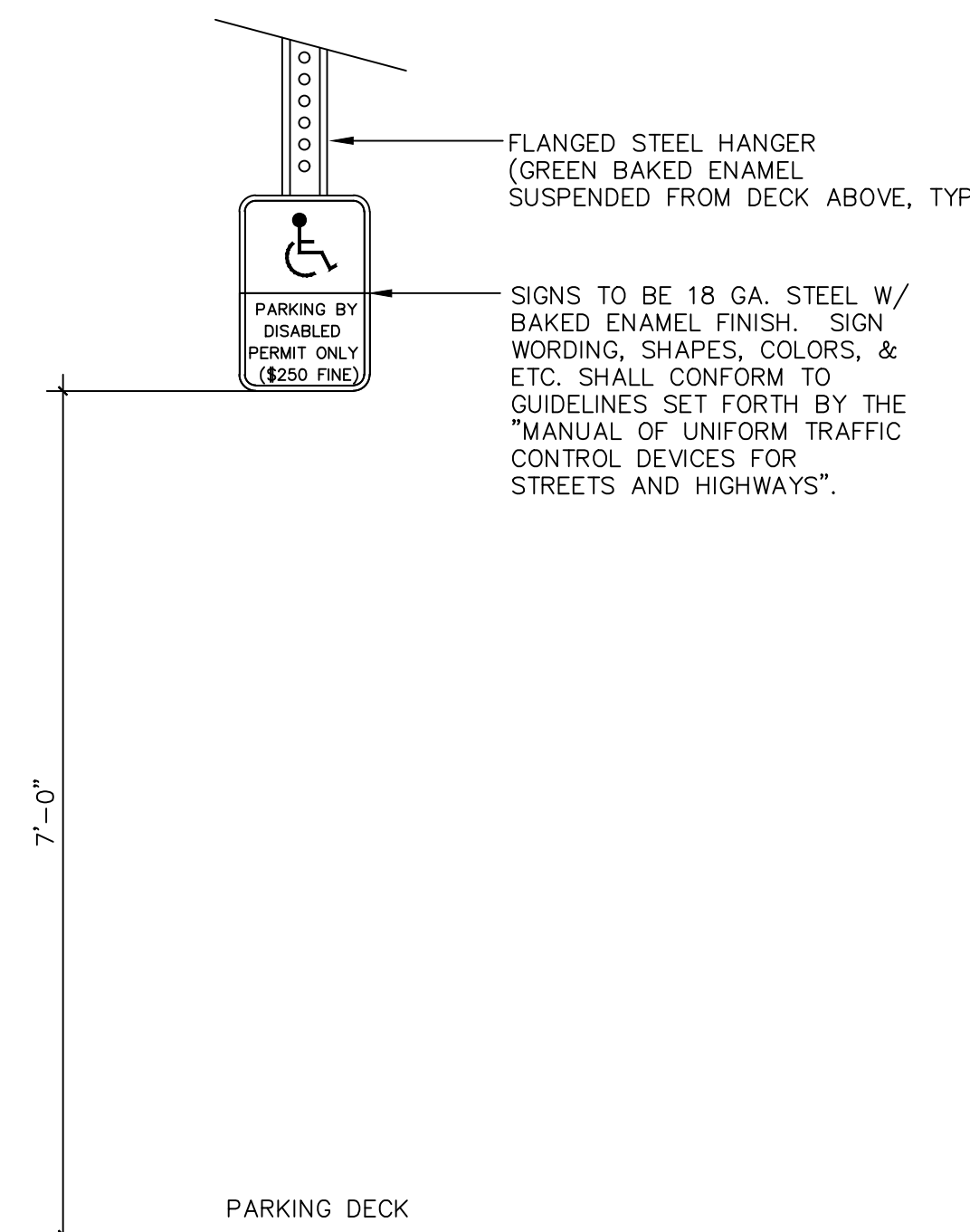
4 H/C SIGN MOUNTING HEIGHT NOT TO SCALE
