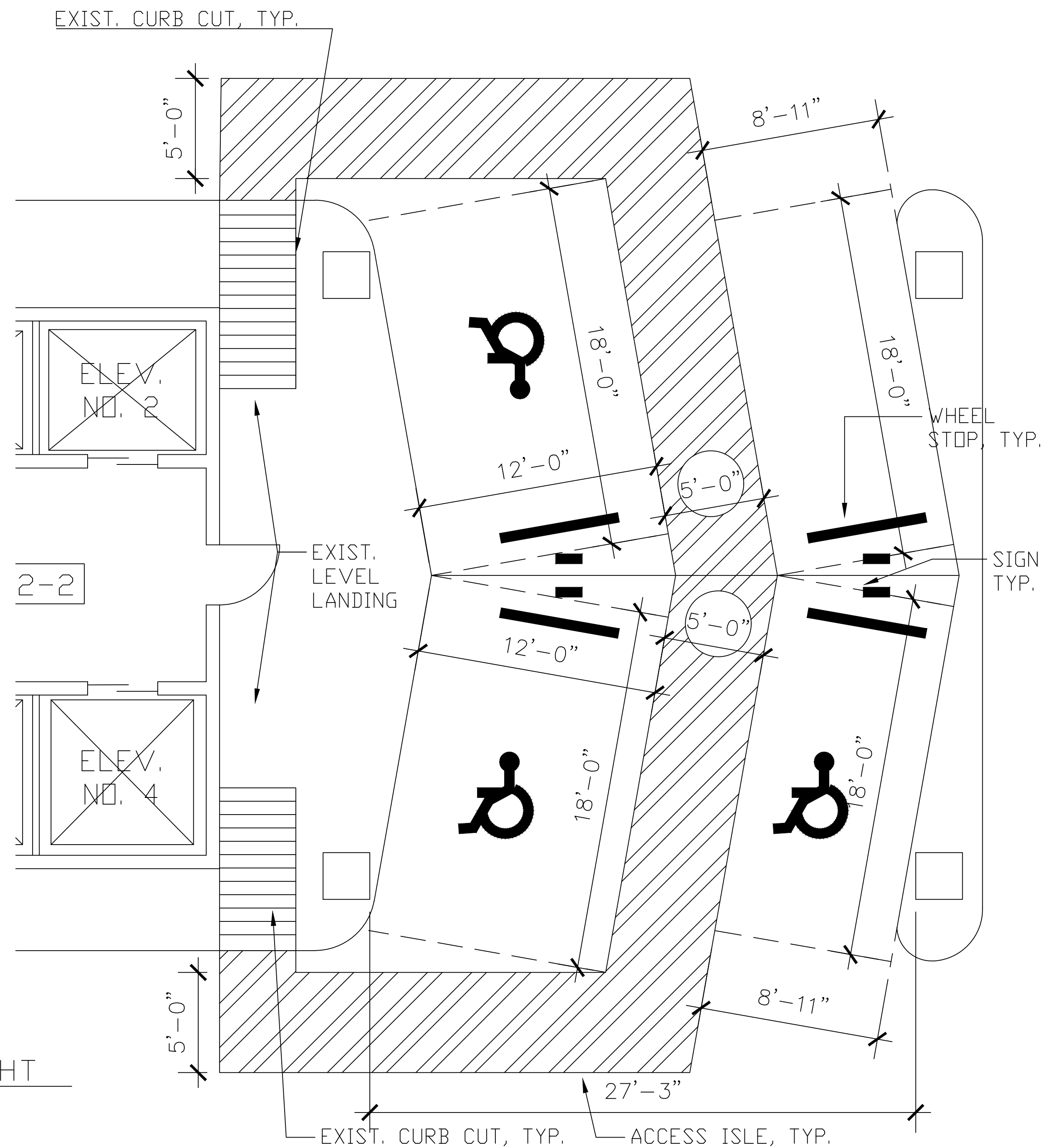
2 ENLARGED PARKING AREA SCALE 1/4"=1'-0"
