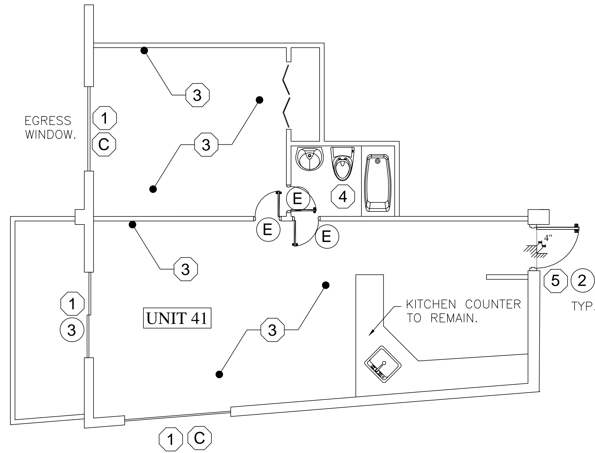
1 ENLARGE UNIT FLOOR PLAN A-1.3.3 SCALE: 1/4" = 1'-0"
