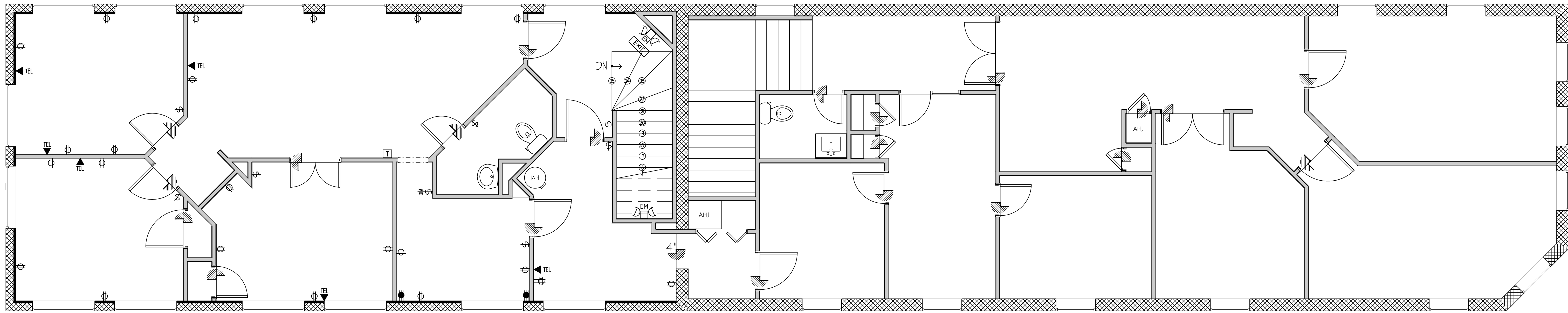
PLAN A-2 EXISTING SECOND FLOOR 1/4" = 1'-0"
