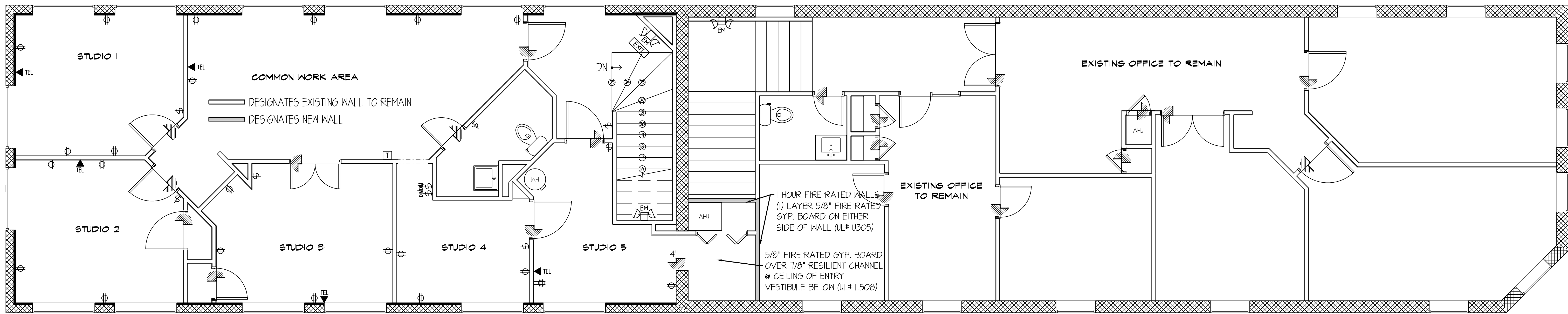
PLAN A-2 PROPOSED SECOND FLOOR 1/4" = 1'-0"
