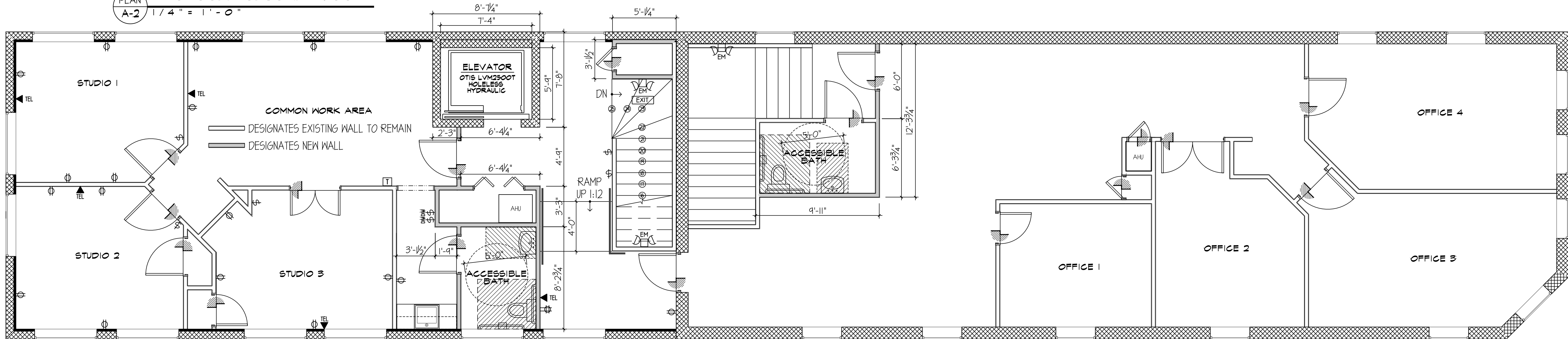
PLAN A-2 ACCESSIBILITY COMPLIANT SECOND FLOOR 1/4" = 1'-0"
