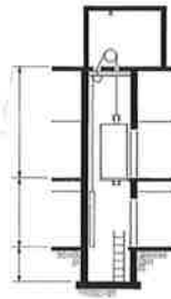
Traction Geared
